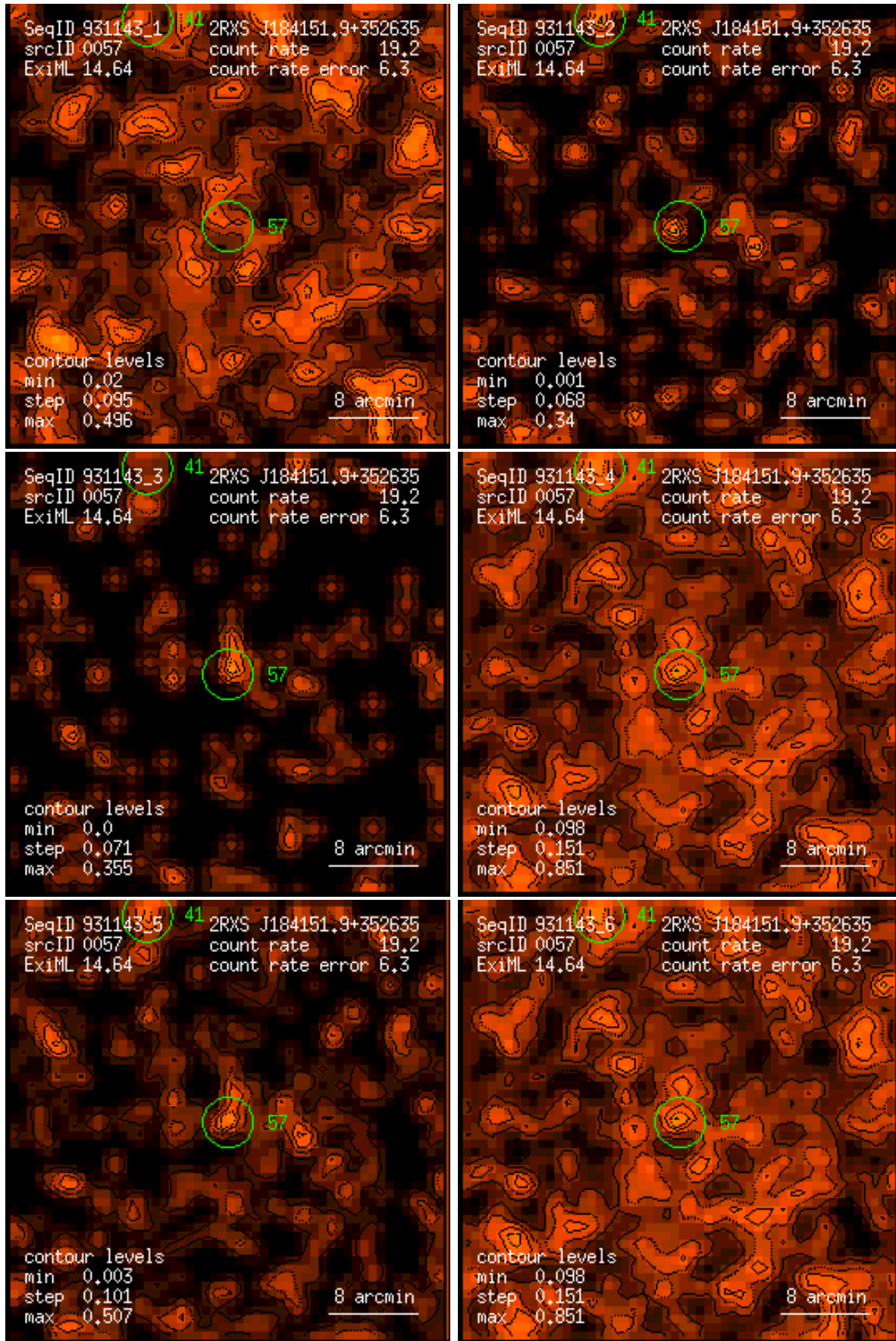
Figure 57: RASS 931143: detection 0057: band rate images, Gaussian filter: (1) PSPC channels 11 – 41, (2) 52 – 90, (3) 91 – 201, (4) 11 – 235, (5) 52 – 201, (6) 11 – 201. Broad band rates in counts/ks. Band rate contour levels in counts/ks/arcmin 2 .
