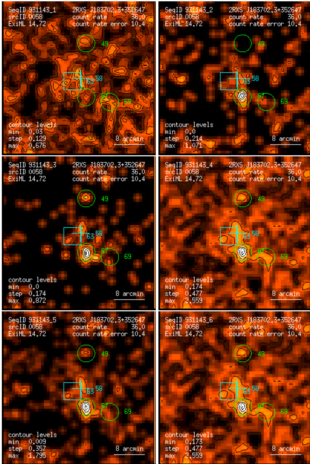
Figure 58: RASS 931143: detection 0058: band rate images, Gaussian filter: (1) PSPC channels 11 – 41, (2) 52 – 90, (3) 91 – 201, (4) 11 – 235, (5) 52 – 201, (6) 11 – 201. Broad band rates in counts/ks. Band rate contour levels in counts/ks/arcmin 2 .
