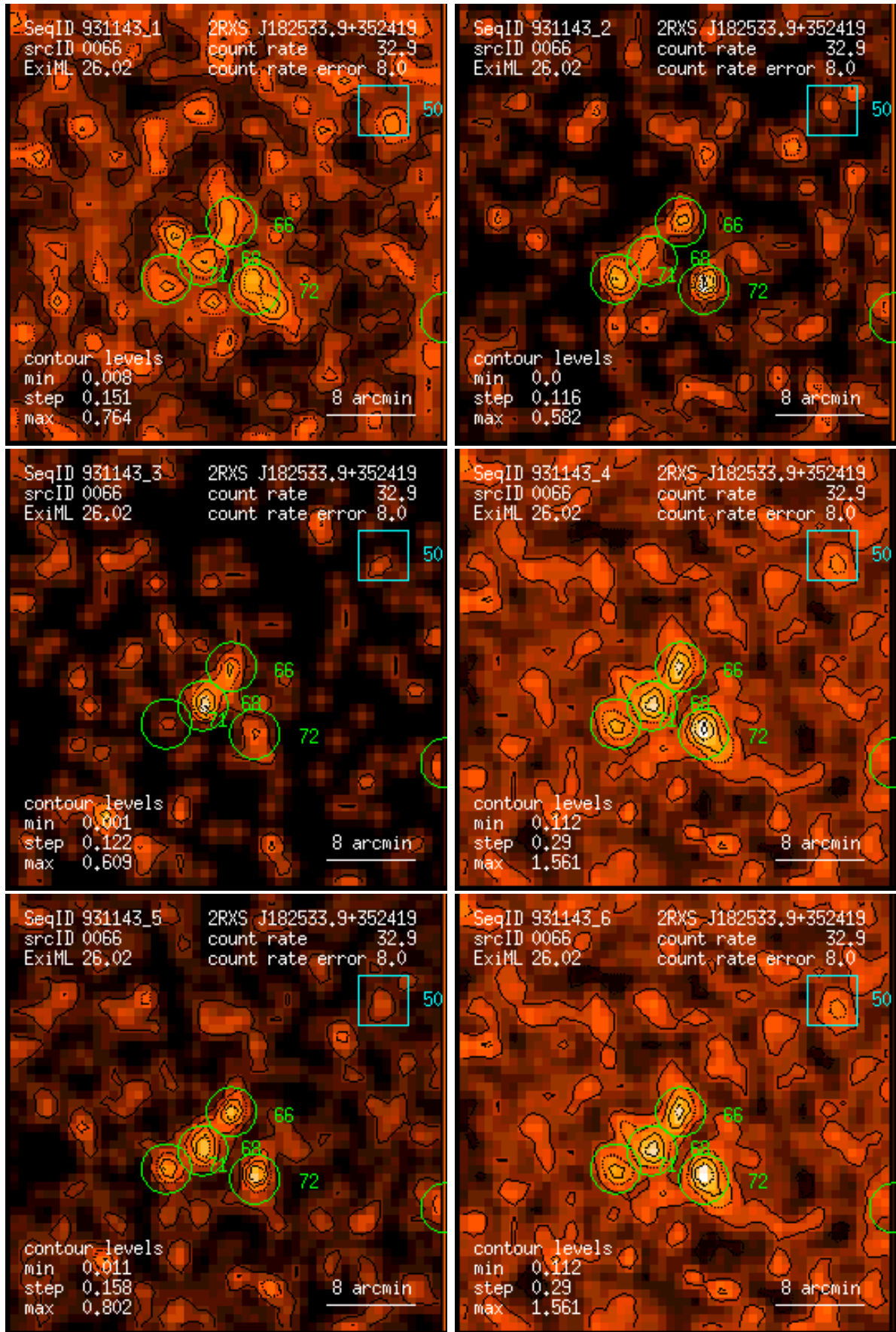
Figure 66: RASS 931143: detection 0066: band rate images, Gaussian filter: (1) PSPC channels 11 – 41, (2) 52 – 90, (3) 91 – 201, (4) 11 – 235, (5) 52 – 201, (6) 11 – 201. Broad band rates in counts/ks. Band rate contour levels in counts/ks/arcmin 2 .
