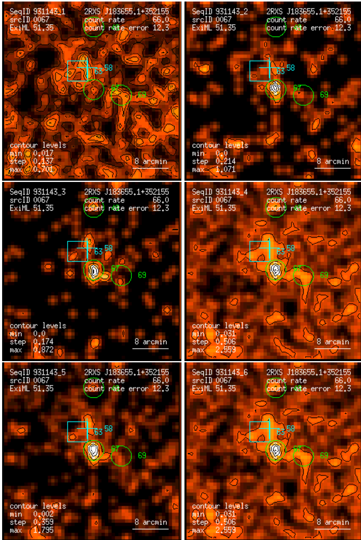
Figure 67: RASS 931143: detection 0067: band rate images, Gaussian filter: (1) PSPC channels 11 – 41, (2) 52 – 90, (3) 91 – 201, (4) 11 – 235, (5) 52 – 201, (6) 11 – 201. Broad band rates in counts/ks. Band rate contour levels in counts/ks/arcmin 2 .
