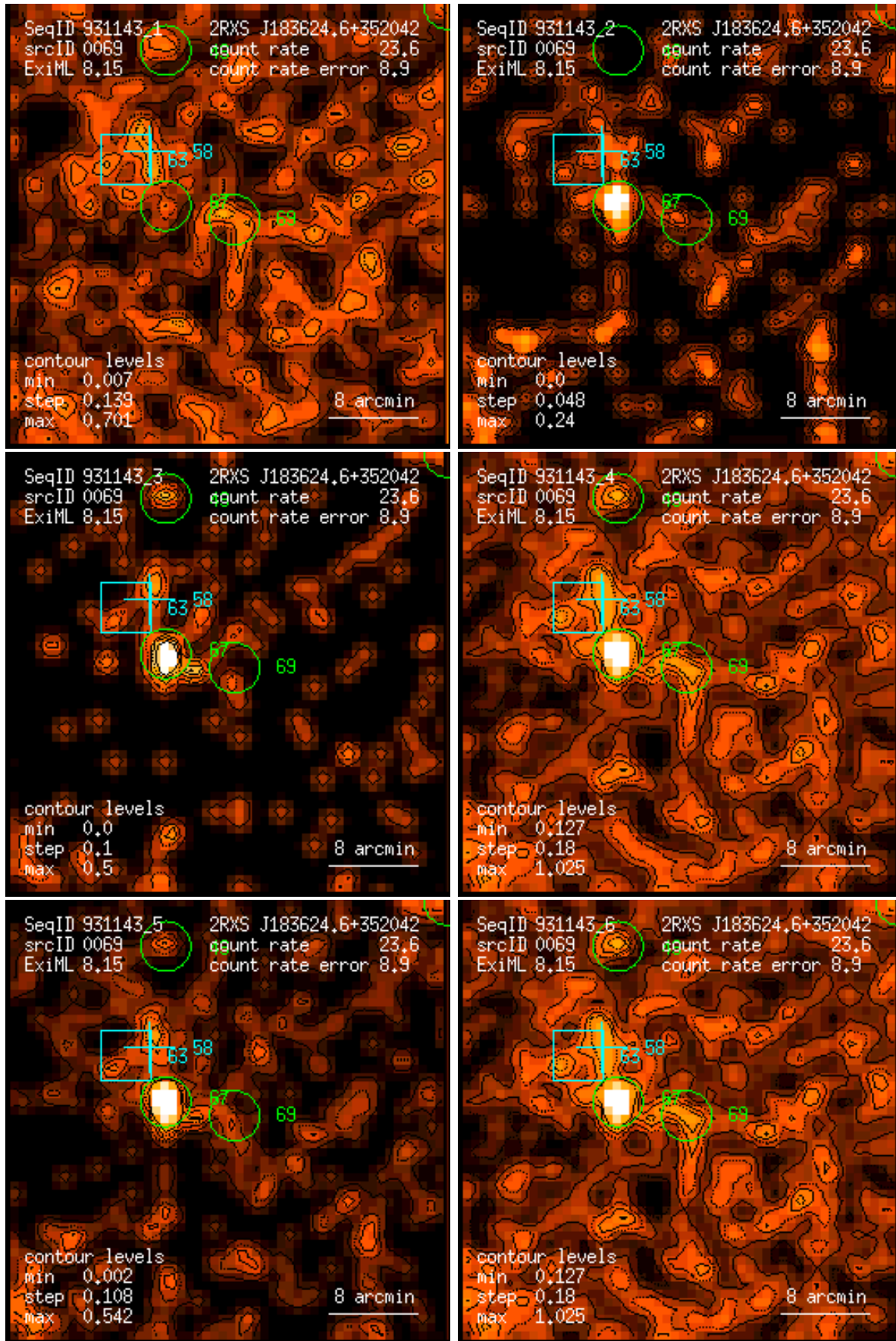
Figure 69: RASS 931143: detection 0069: band rate images, Gaussian filter: (1) PSPC channels 11 – 41, (2) 52 – 90, (3) 91 – 201, (4) 11 – 235, (5) 52 – 201, (6) 11 – 201. Broad band rates in counts/ks. Band rate contour levels in counts/ks/arcmin 2 .
