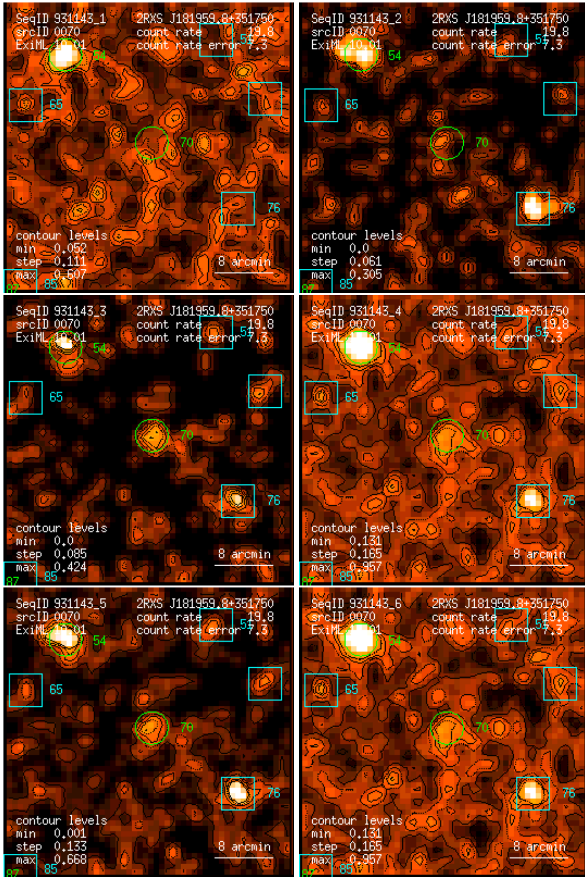
Figure 70: RASS 931143: detection 0070: band rate images, Gaussian filter: (1) PSPC channels 11 – 41, (2) 52 – 90, (3) 91 – 201, (4) 11 – 235, (5) 52 – 201, (6) 11 – 201. Broad band rates in counts/ks. Band rate contour levels in counts/ks/arcmin 2 .
