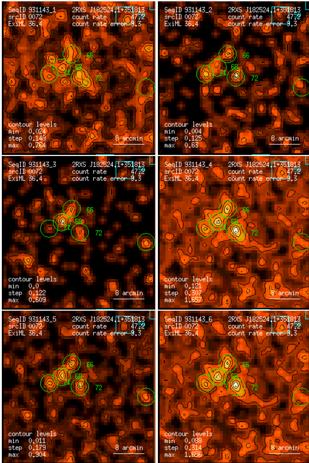
Figure 72: RASS 931143: detection 0072: band rate images, Gaussian filter: (1) PSPC channels 11 – 41, (2) 52 – 90, (3) 91 – 201, (4) 11 – 235, (5) 52 – 201, (6) 11 – 201. Broad band rates in counts/ks. Band rate contour levels in counts/ks/arcmin 2 .
