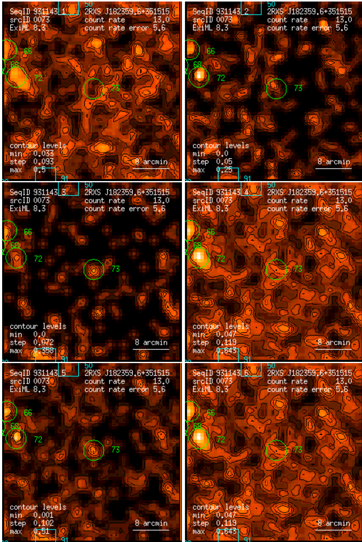
Figure 73: RASS 931143: detection 0073: band rate images, Gaussian filter: (1) PSPC channels 11 – 41, (2) 52 – 90, (3) 91 – 201, (4) 11 – 235, (5) 52 – 201, (6) 11 – 201. Broad band rates in counts/ks. Band rate contour levels in counts/ks/arcmin 2 .
