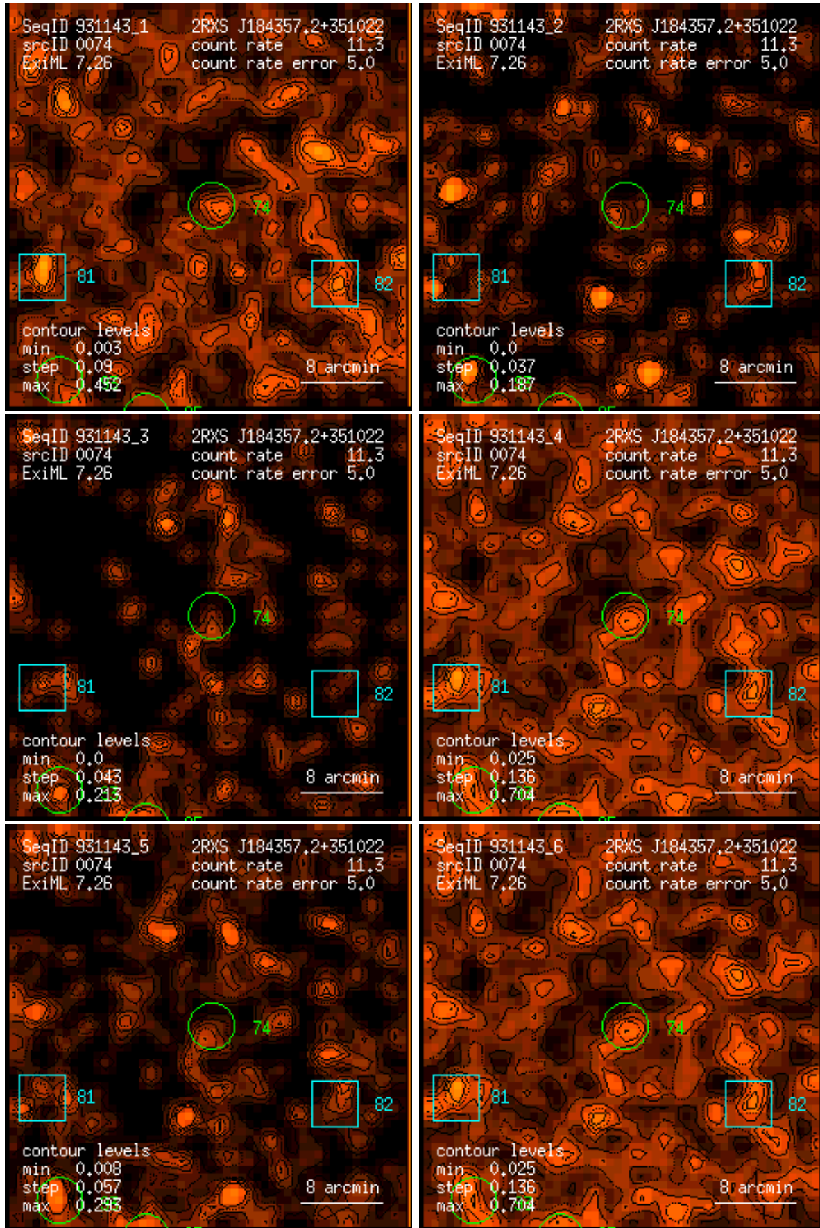
Figure 74: RASS 931143: detection 0074: band rate images, Gaussian filter: (1) PSPC channels 11 – 41, (2) 52 – 90, (3) 91 – 201, (4) 11 – 235, (5) 52 – 201, (6) 11 – 201. Broad band rates in counts/ks. Band rate contour levels in counts/ks/arcmin 2 .
