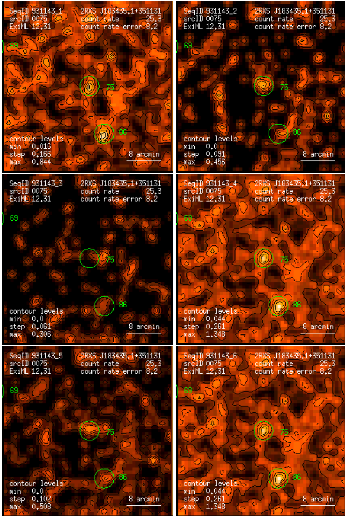
Figure 75: RASS 931143: detection 0075: band rate images, Gaussian filter: (1) PSPC channels 11 – 41, (2) 52 – 90, (3) 91 – 201, (4) 11 – 235, (5) 52 – 201, (6) 11 – 201. Broad band rates in counts/ks. Band rate contour levels in counts/ks/arcmin 2 .
