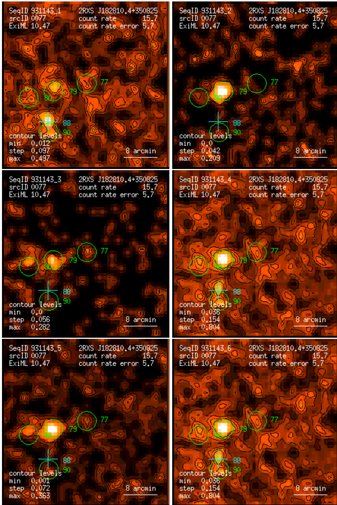
Figure 77: RASS 931143: detection 0077: band rate images, Gaussian filter: (1) PSPC channels 11 – 41, (2) 52 – 90, (3) 91 – 201, (4) 11 – 235, (5) 52 – 201, (6) 11 – 201. Broad band rates in counts/ks. Band rate contour levels in counts/ks/arcmin 2 .
