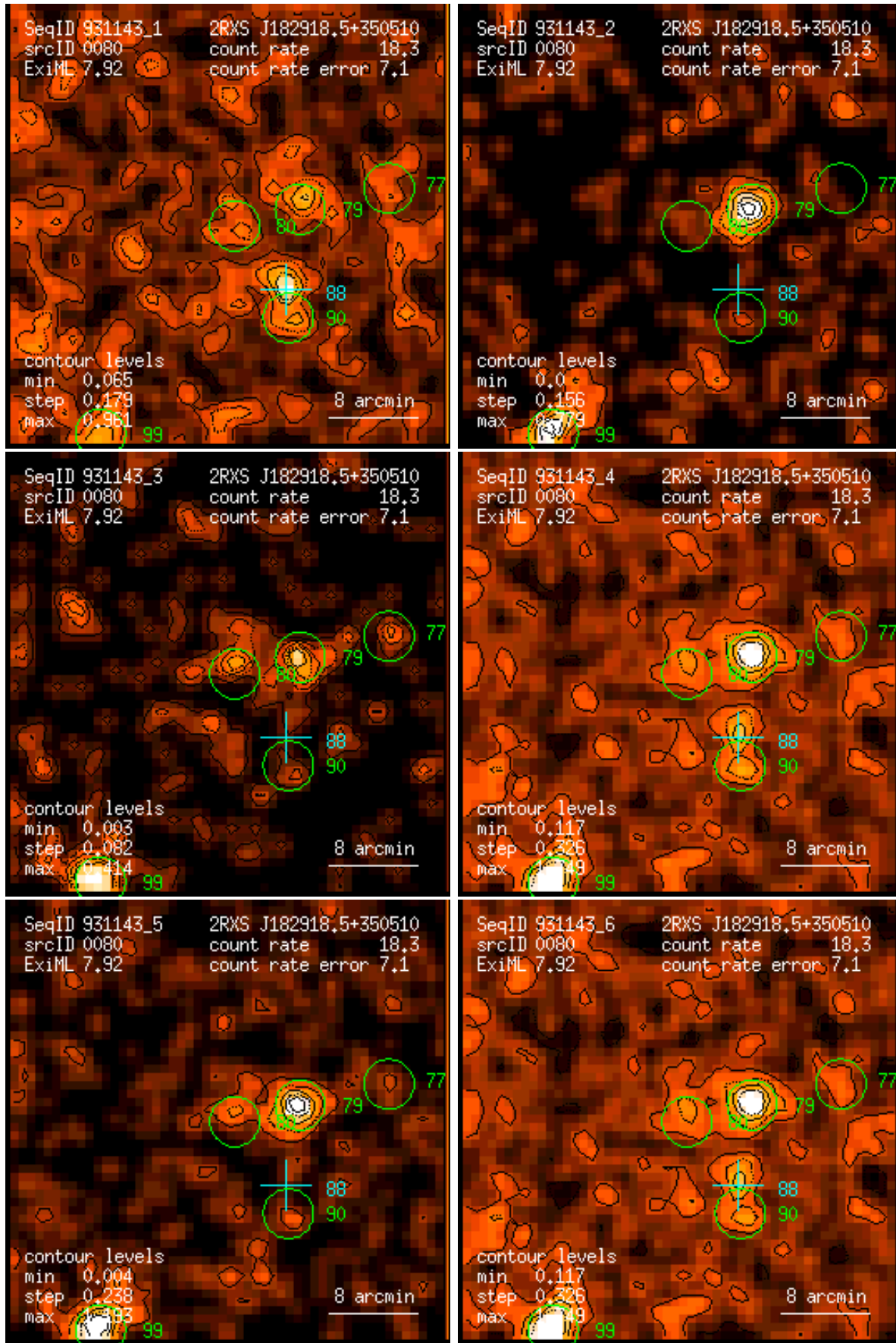
Figure 80: RASS 931143: detection 0080: band rate images, Gaussian filter: (1) PSPC channels 11 – 41, (2) 52 – 90, (3) 91 – 201, (4) 11 – 235, (5) 52 – 201, (6) 11 – 201. Broad band rates in counts/ks. Band rate contour levels in counts/ks/arcmin 2 .
