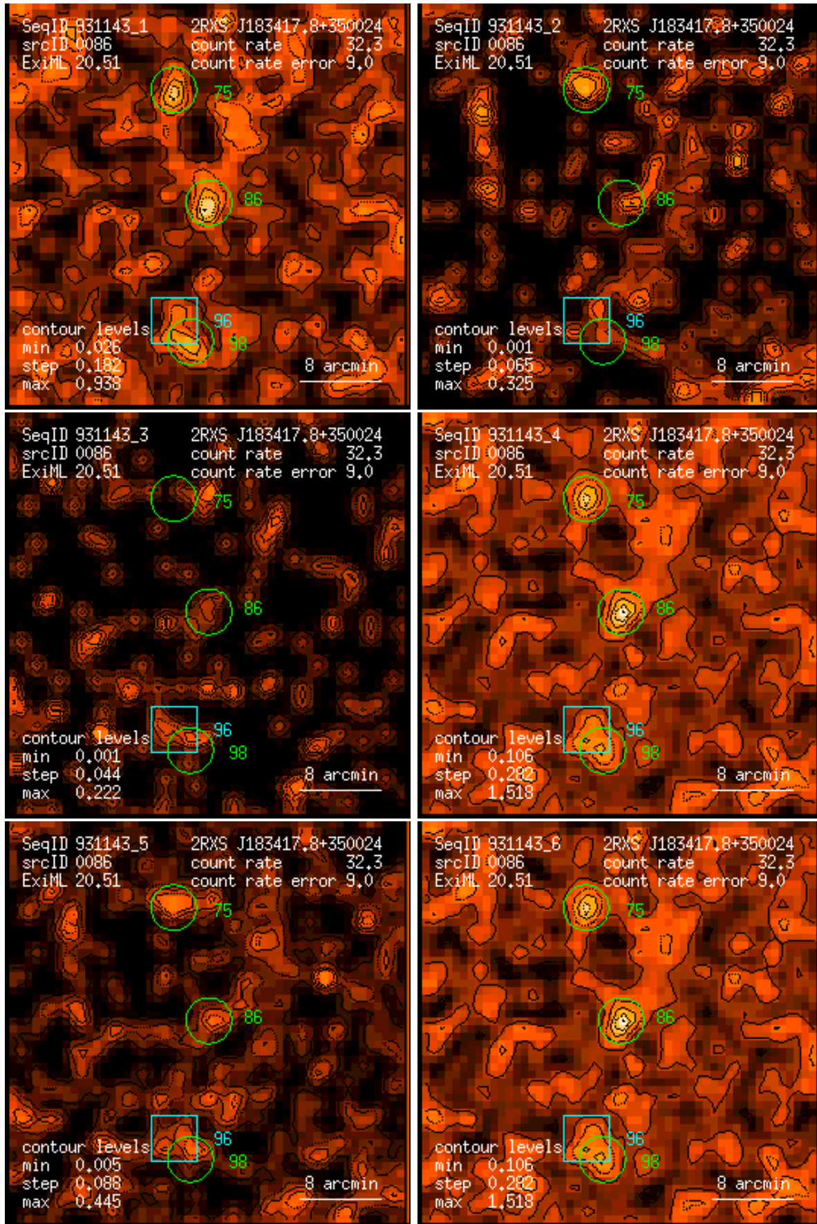
Figure 86: RASS 931143: detection 0086: band rate images, Gaussian filter: (1) PSPC channels 11 – 41, (2) 52 – 90, (3) 91 – 201, (4) 11 – 235, (5) 52 – 201, (6) 11 – 201. Broad band rates in counts/ks. Band rate contour levels in counts/ks/arcmin 2 .
