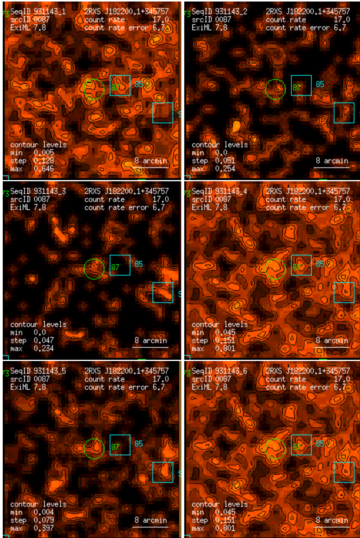
Figure 87: RASS 931143: detection 0087: band rate images, Gaussian filter: (1) PSPC channels 11 – 41, (2) 52 – 90, (3) 91 – 201, (4) 11 – 235, (5) 52 – 201, (6) 11 – 201. Broad band rates in counts/ks. Band rate contour levels in counts/ks/arcmin 2 .
