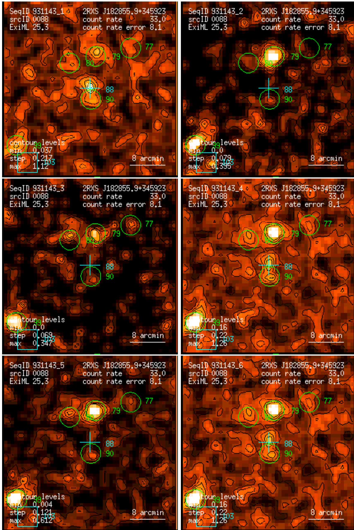
Figure 88: RASS 931143: detection 0088: band rate images, Gaussian filter: (1) PSPC channels 11 – 41, (2) 52 – 90, (3) 91 – 201, (4) 11 – 235, (5) 52 – 201, (6) 11 – 201. Broad band rates in counts/ks. Band rate contour levels in counts/ks/arcmin 2 .
