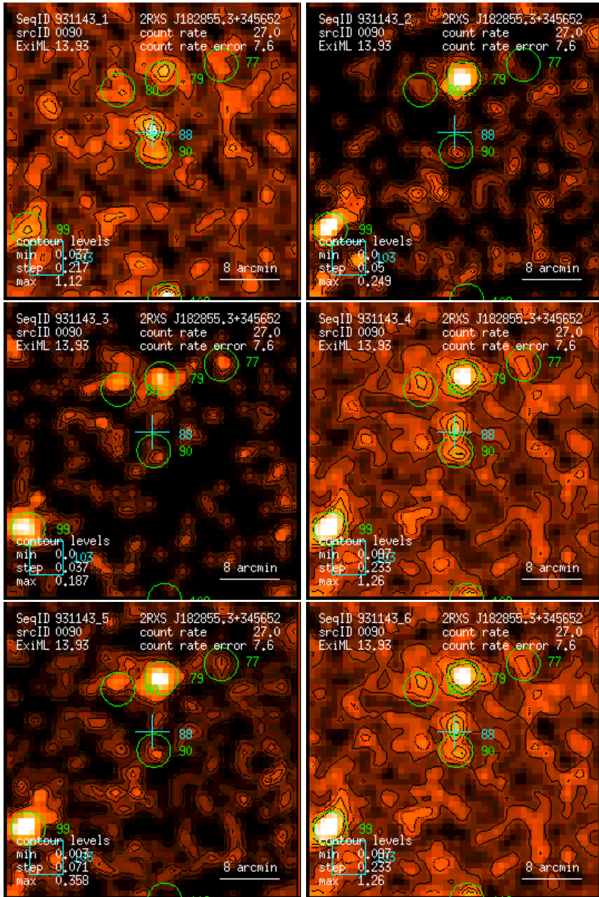
Figure 90: RASS 931143: detection 0090: band rate images, Gaussian filter: (1) PSPC channels 11 – 41, (2) 52 – 90, (3) 91 – 201, (4) 11 – 235, (5) 52 – 201, (6) 11 – 201. Broad band rates in counts/ks. Band rate contour levels in counts/ks/arcmin 2 .
