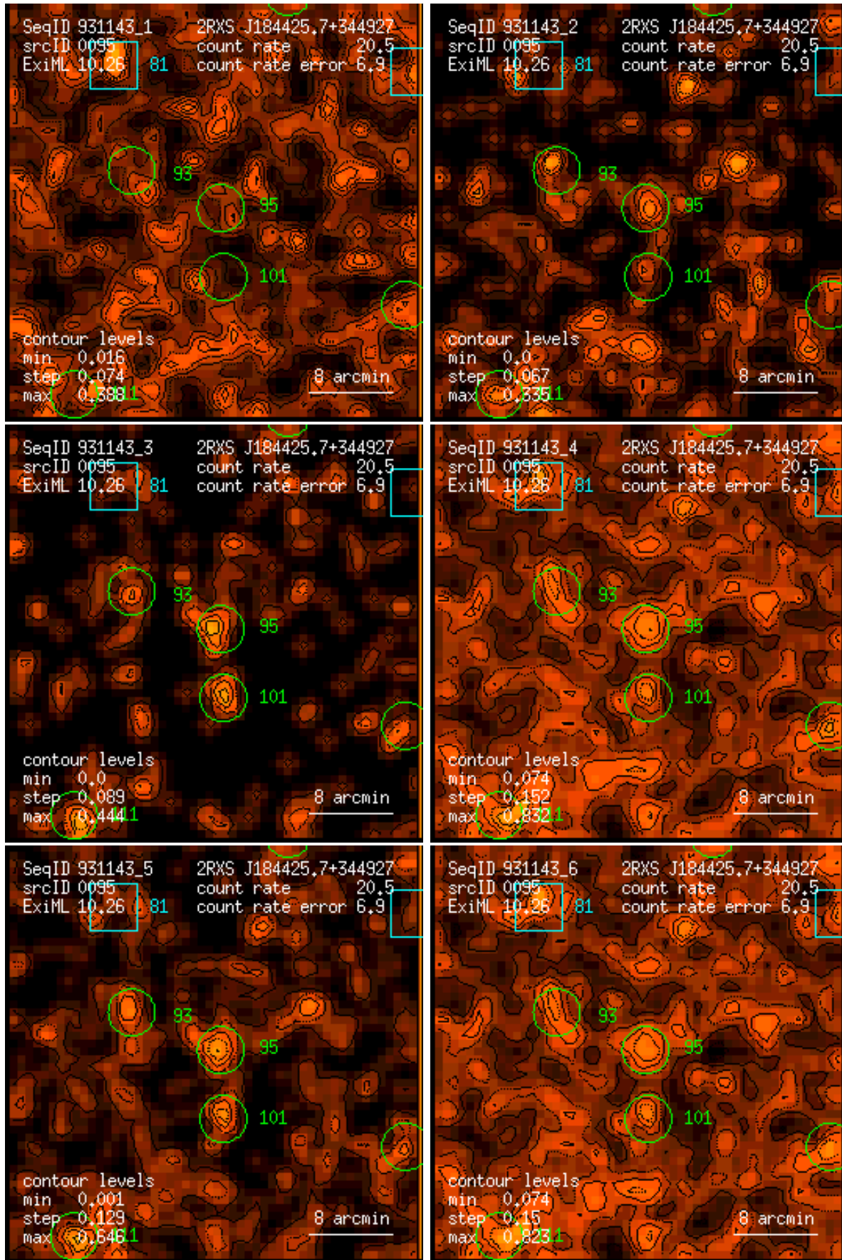
Figure 95: RASS 931143: detection 0095: band rate images, Gaussian filter: (1) PSPC channels 11 – 41, (2) 52 – 90, (3) 91 – 201, (4) 11 – 235, (5) 52 – 201, (6) 11 – 201. Broad band rates in counts/ks. Band rate contour levels in counts/ks/arcmin 2 .
