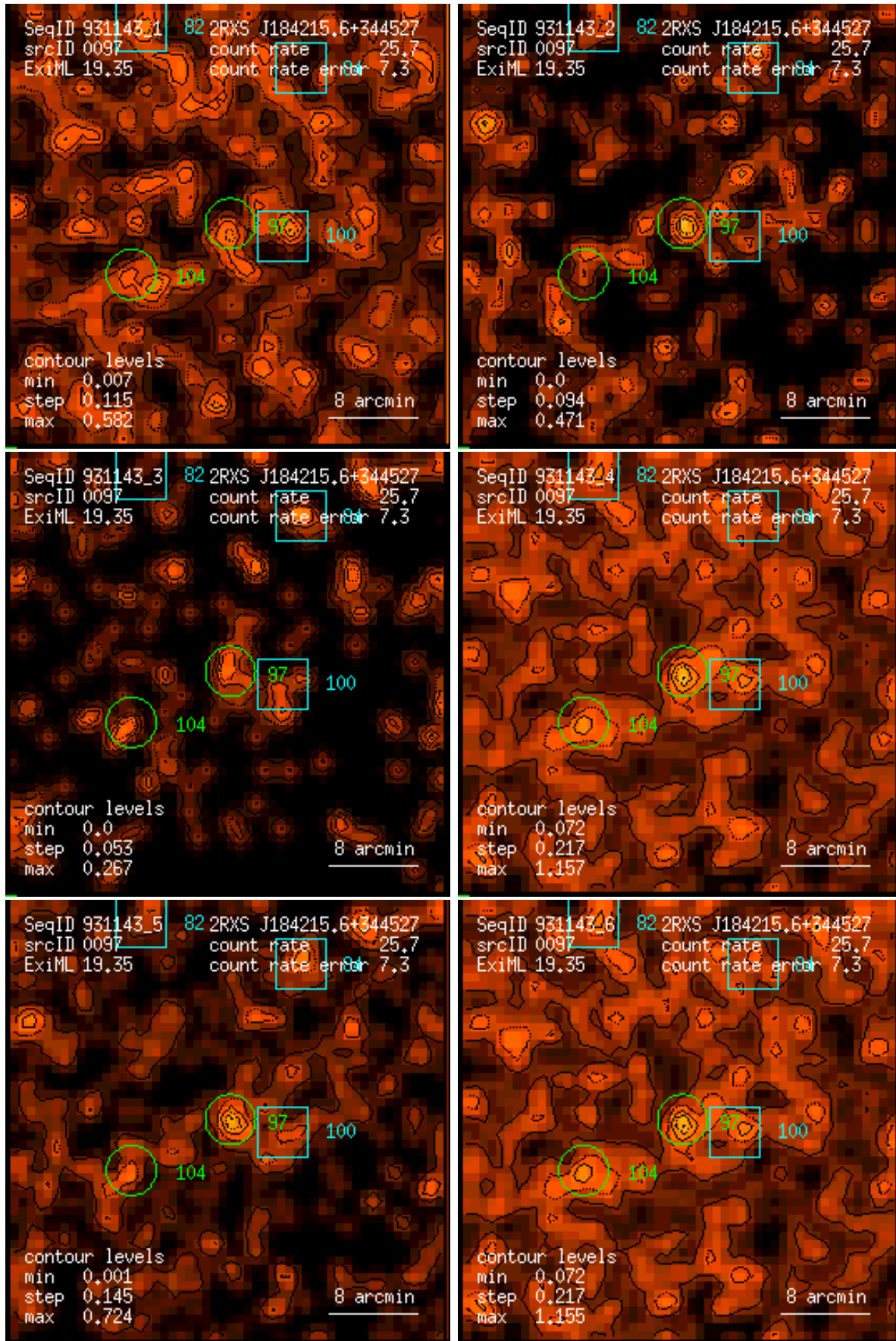
Figure 97: RASS 931143: detection 0097: band rate images, Gaussian filter: (1) PSPC channels 11 – 41, (2) 52 – 90, (3) 91 – 201, (4) 11 – 235, (5) 52 – 201, (6) 11 – 201. Broad band rates in counts/ks. Band rate contour levels in counts/ks/arcmin 2 .
