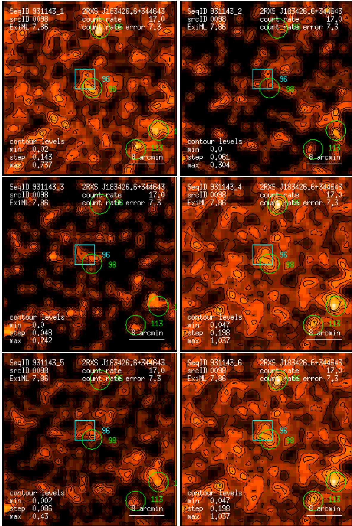
Figure 98: RASS 931143: detection 0098: band rate images, Gaussian filter: (1) PSPC channels 11 – 41, (2) 52 – 90, (3) 91 – 201, (4) 11 – 235, (5) 52 – 201, (6) 11 – 201. Broad band rates in counts/ks. Band rate contour levels in counts/ks/arcmin 2 .
