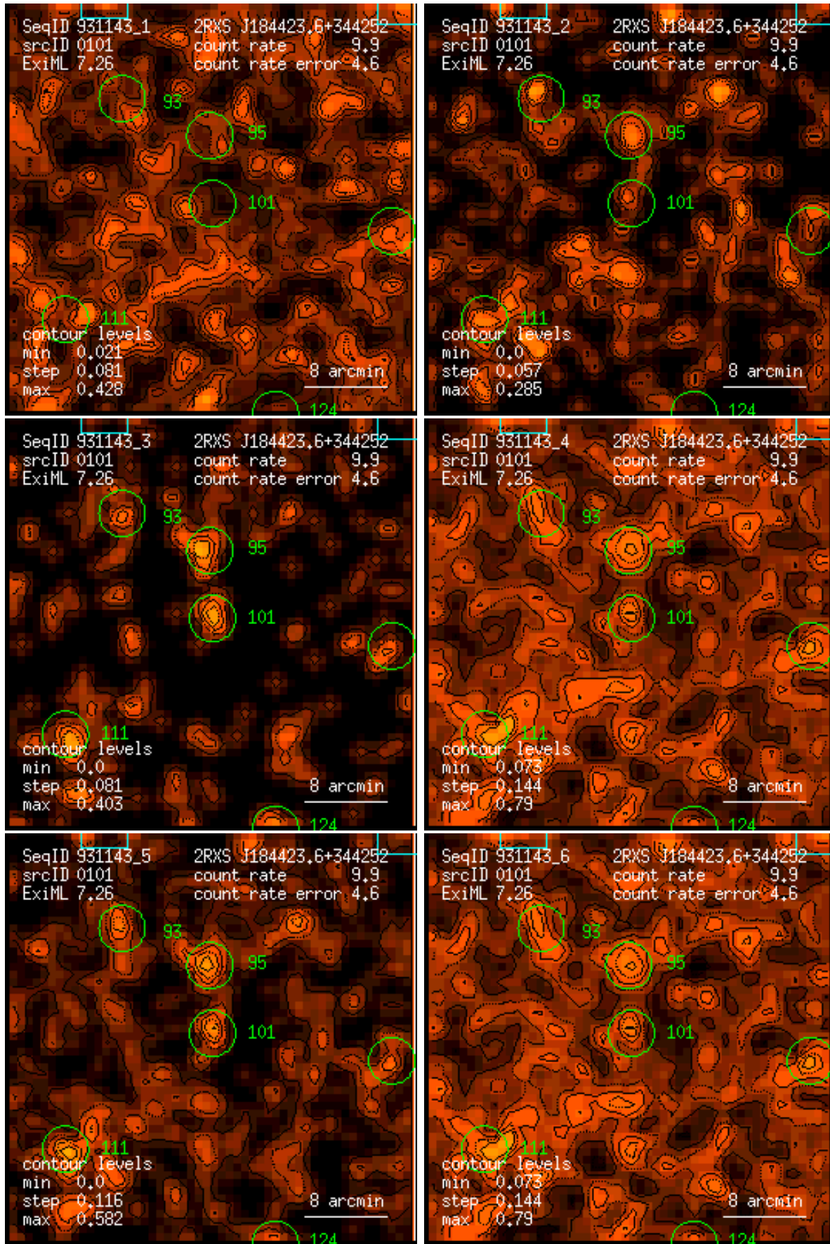
Figure 101: RASS 931143: detection 0101: band rate images, Gaussian filter: (1) PSPC channels 11 – 41, (2) 52 – 90, (3) 91 – 201, (4) 11 – 235, (5) 52 – 201, (6) 11 – 201. Broad band rates in counts/ks. Band rate contour levels in counts/ks/arcmin 2 .
