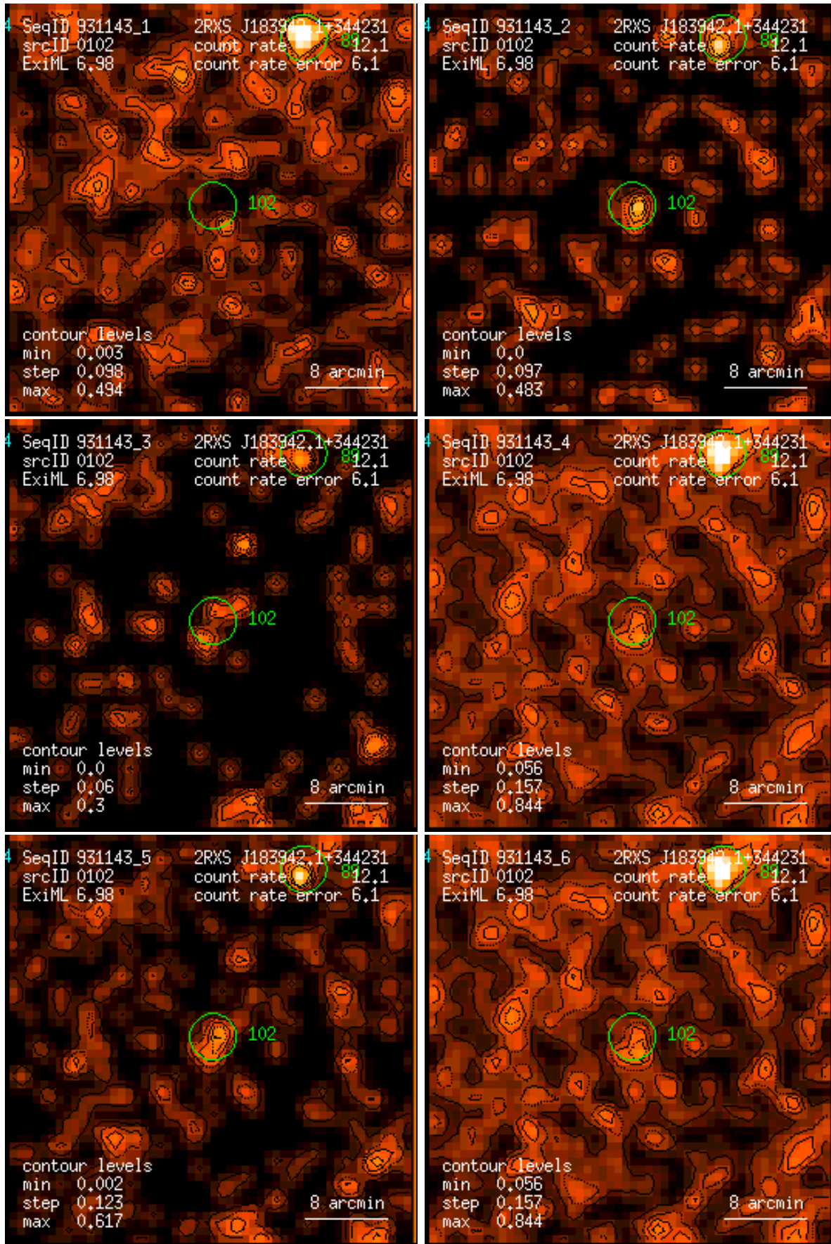
Figure 102: RASS 931143: detection 0102: band rate images, Gaussian filter: (1) PSPC channels 11 – 41, (2) 52 – 90, (3) 91 – 201, (4) 11 – 235, (5) 52 – 201, (6) 11 – 201. Broad band rates in counts/ks. Band rate contour levels in counts/ks/arcmin 2 .
