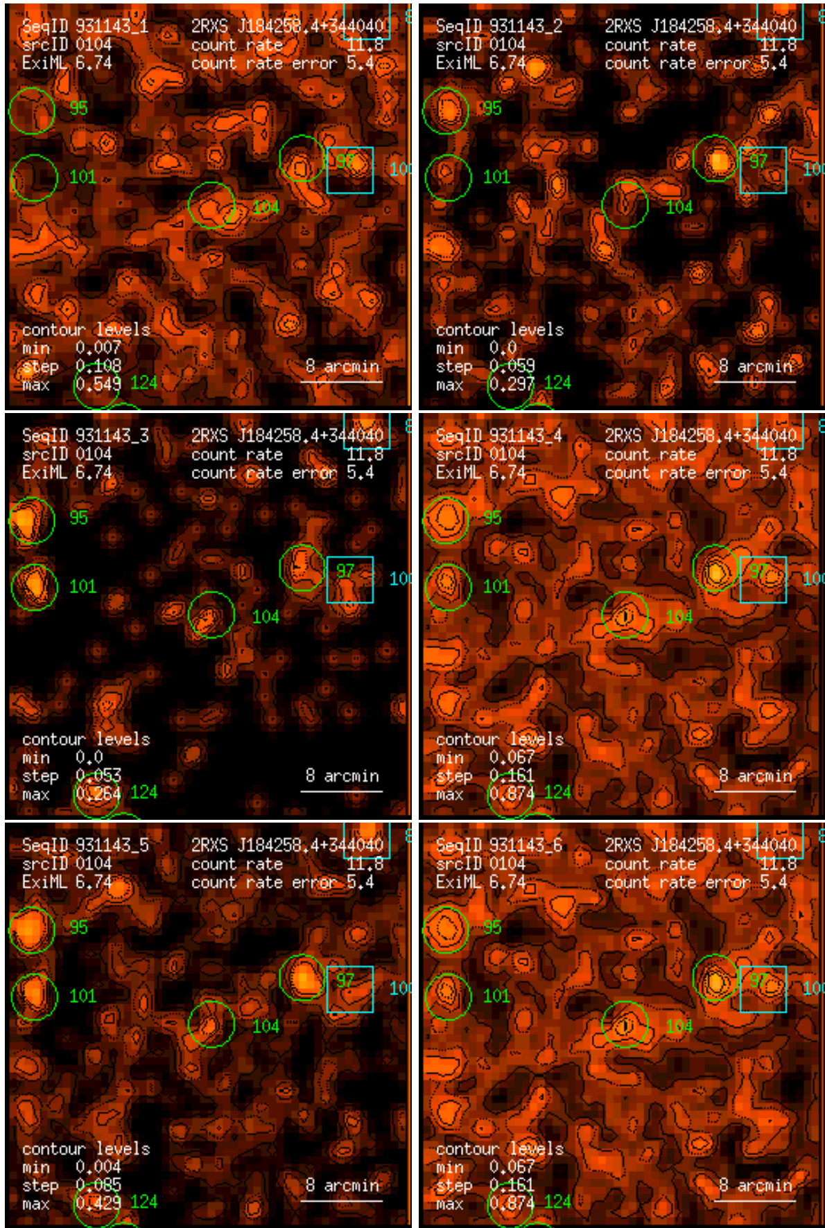
Figure 104: RASS 931143: detection 0104: band rate images, Gaussian filter: (1) PSPC channels 11 – 41, (2) 52 – 90, (3) 91 – 201, (4) 11 – 235, (5) 52 – 201, (6) 11 – 201. Broad band rates in counts/ks. Band rate contour levels in counts/ks/arcmin 2 .
