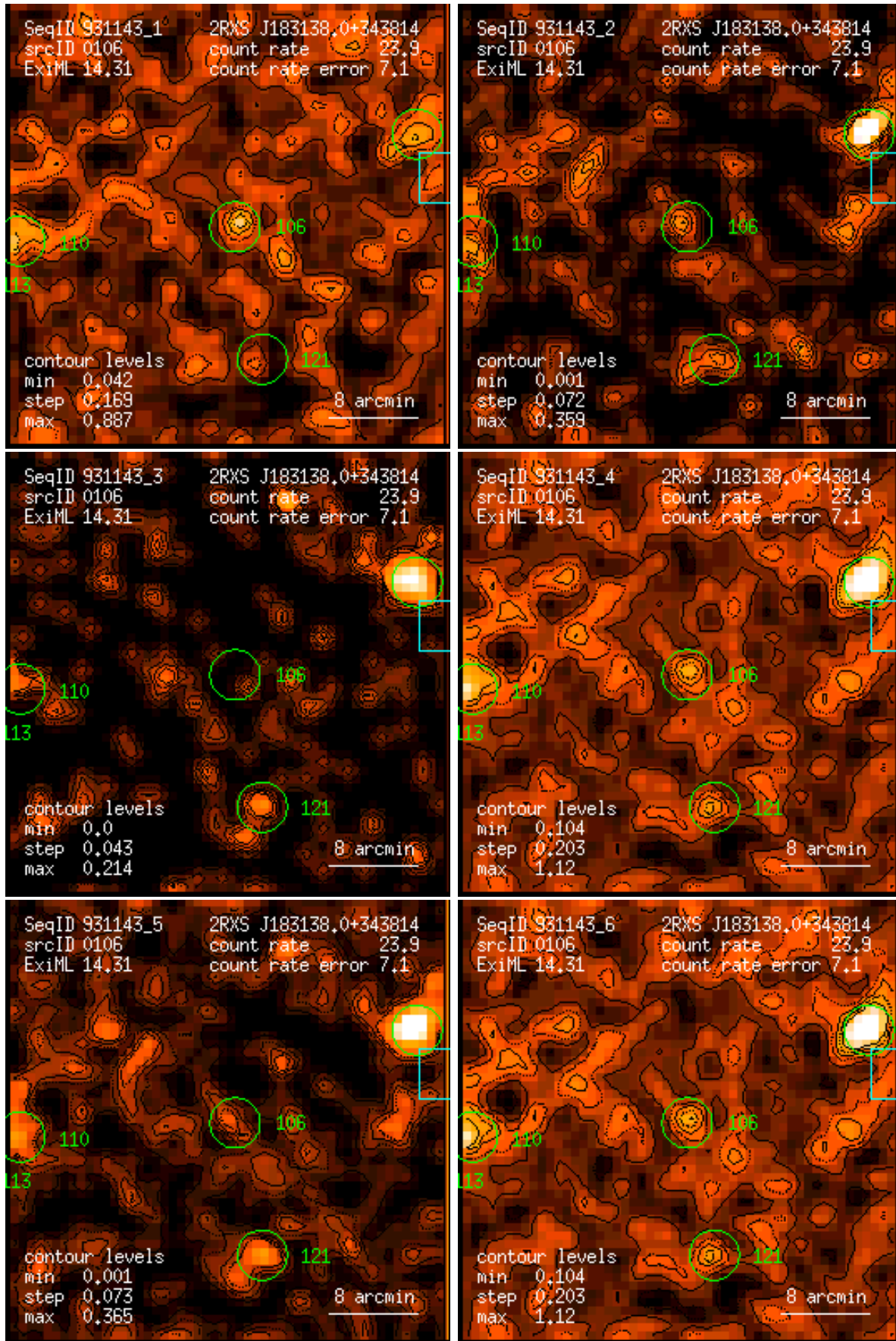
Figure 106: RASS 931143: detection 0106: band rate images, Gaussian filter: (1) PSPC channels 11 – 41, (2) 52 – 90, (3) 91 – 201, (4) 11 – 235, (5) 52 – 201, (6) 11 – 201. Broad band rates in counts/ks. Band rate contour levels in counts/ks/arcmin 2 .
