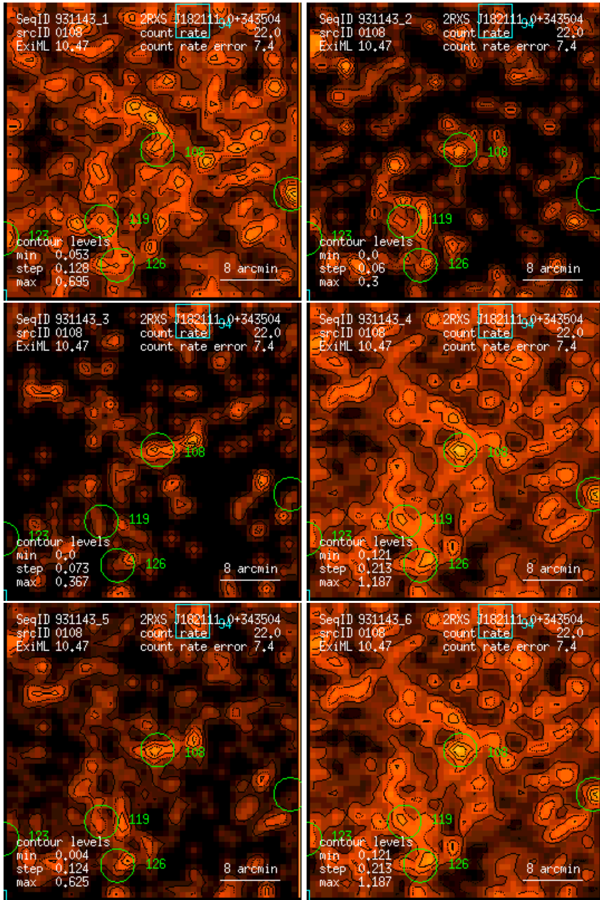
Figure 108: RASS 931143: detection 0108: band rate images, Gaussian filter: (1) PSPC channels 11 – 41, (2) 52 – 90, (3) 91 – 201, (4) 11 – 235, (5) 52 – 201, (6) 11 – 201. Broad band rates in counts/ks. Band rate contour levels in counts/ks/arcmin 2 .
