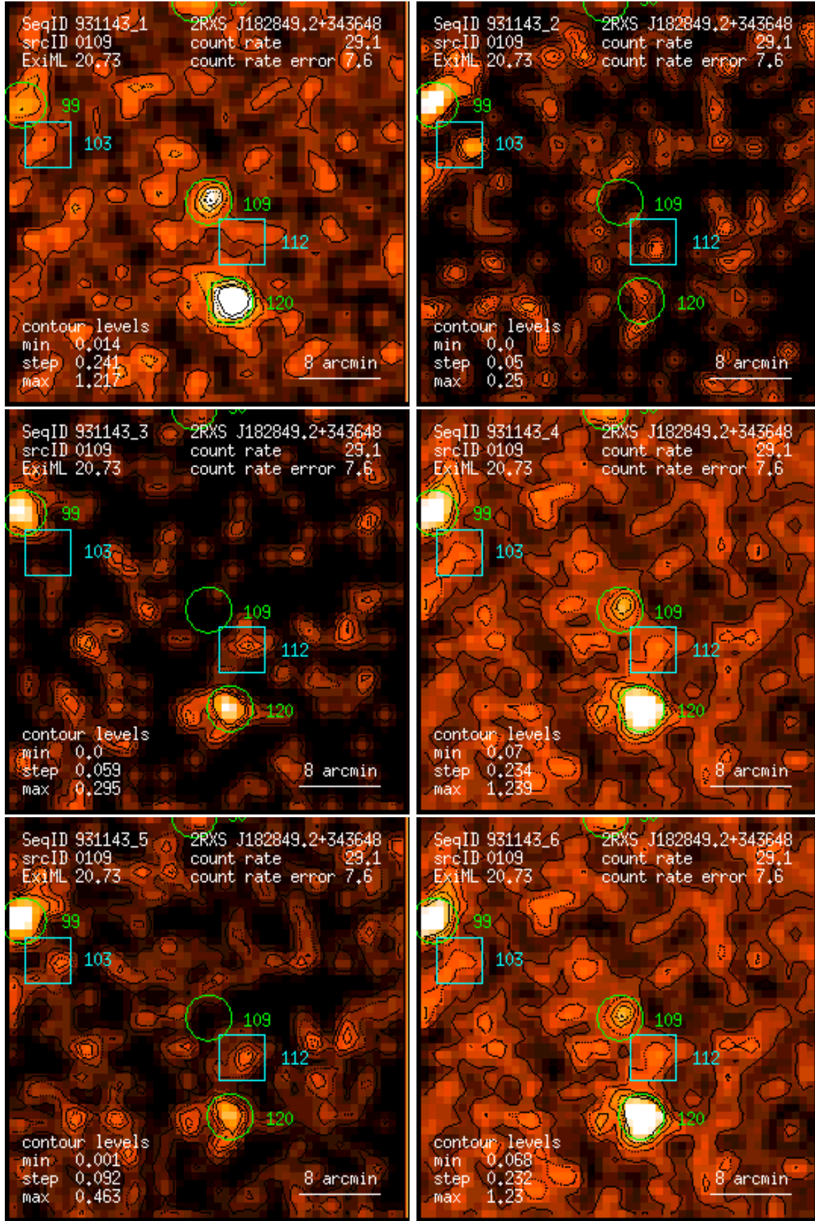
Figure 109: RASS 931143: detection 0109: band rate images, Gaussian filter: (1) PSPC channels 11 – 41, (2) 52 – 90, (3) 91 – 201, (4) 11 – 235, (5) 52 – 201, (6) 11 – 201. Broad band rates in counts/ks. Band rate contour levels in counts/ks/arcmin 2 .
