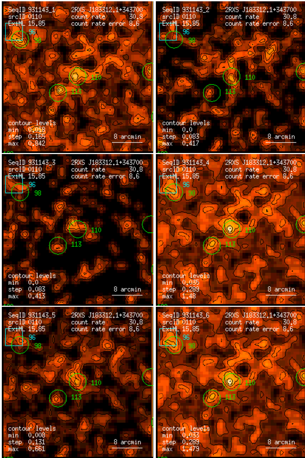
Figure 110: RASS 931143: detection 0110: band rate images, Gaussian filter: (1) PSPC channels 11 – 41, (2) 52 – 90, (3) 91 – 201, (4) 11 – 235, (5) 52 – 201, (6) 11 – 201. Broad band rates in counts/ks. Band rate contour levels in counts/ks/arcmin 2 .
