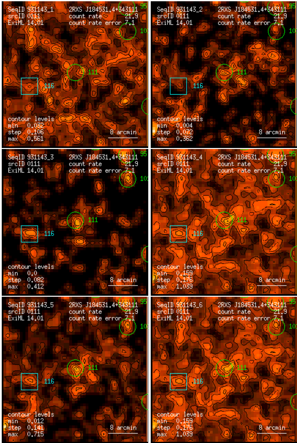
Figure 111: RASS 931143: detection 0111: band rate images, Gaussian filter: (1) PSPC channels 11 – 41, (2) 52 – 90, (3) 91 – 201, (4) 11 – 235, (5) 52 – 201, (6) 11 – 201. Broad band rates in counts/ks. Band rate contour levels in counts/ks/arcmin 2 .
