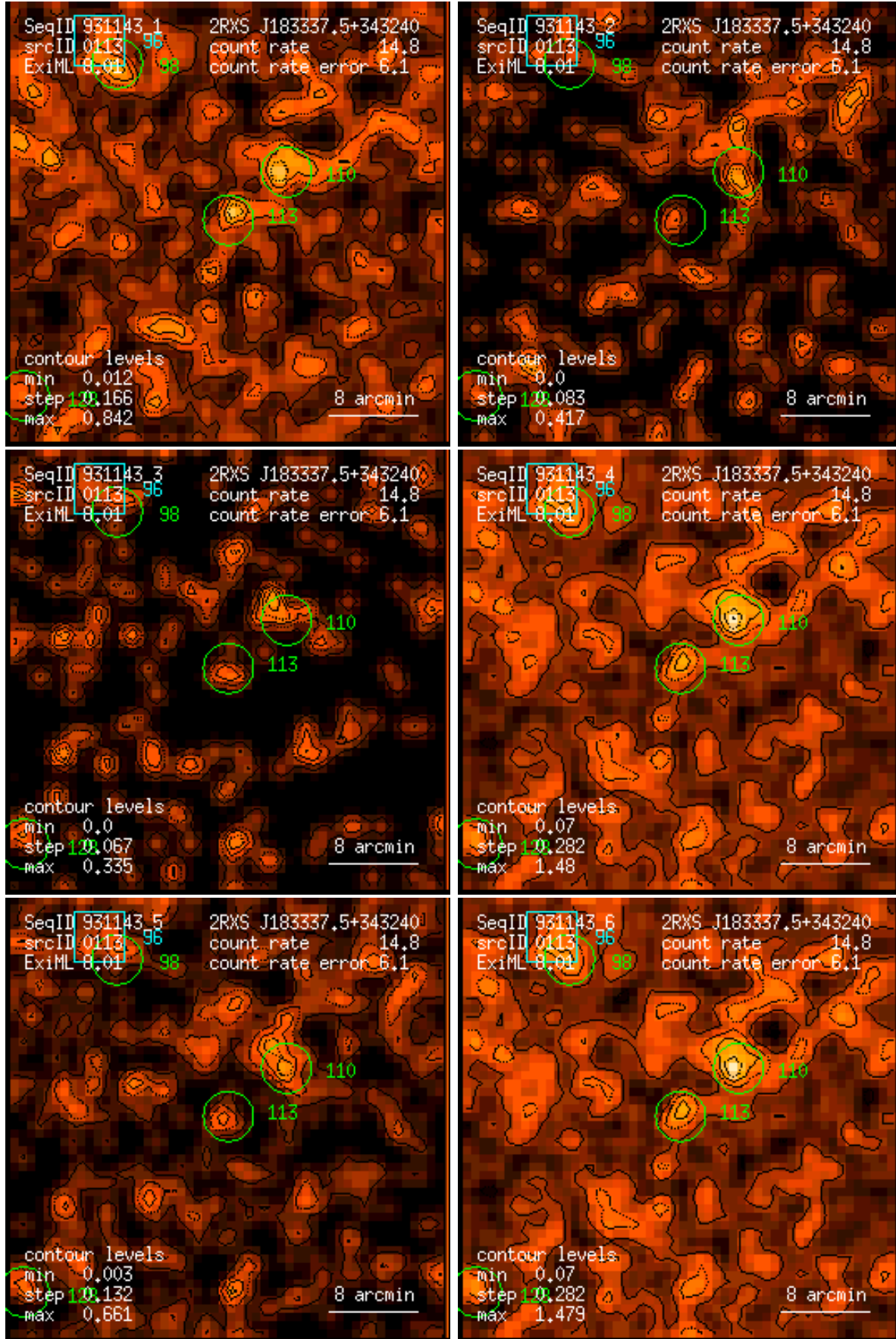
Figure 113: RASS 931143: detection 0113: band rate images, Gaussian filter: (1) PSPC channels 11 – 41, (2) 52 – 90, (3) 91 – 201, (4) 11 – 235, (5) 52 – 201, (6) 11 – 201. Broad band rates in counts/ks. Band rate contour levels in counts/ks/arcmin 2 .
