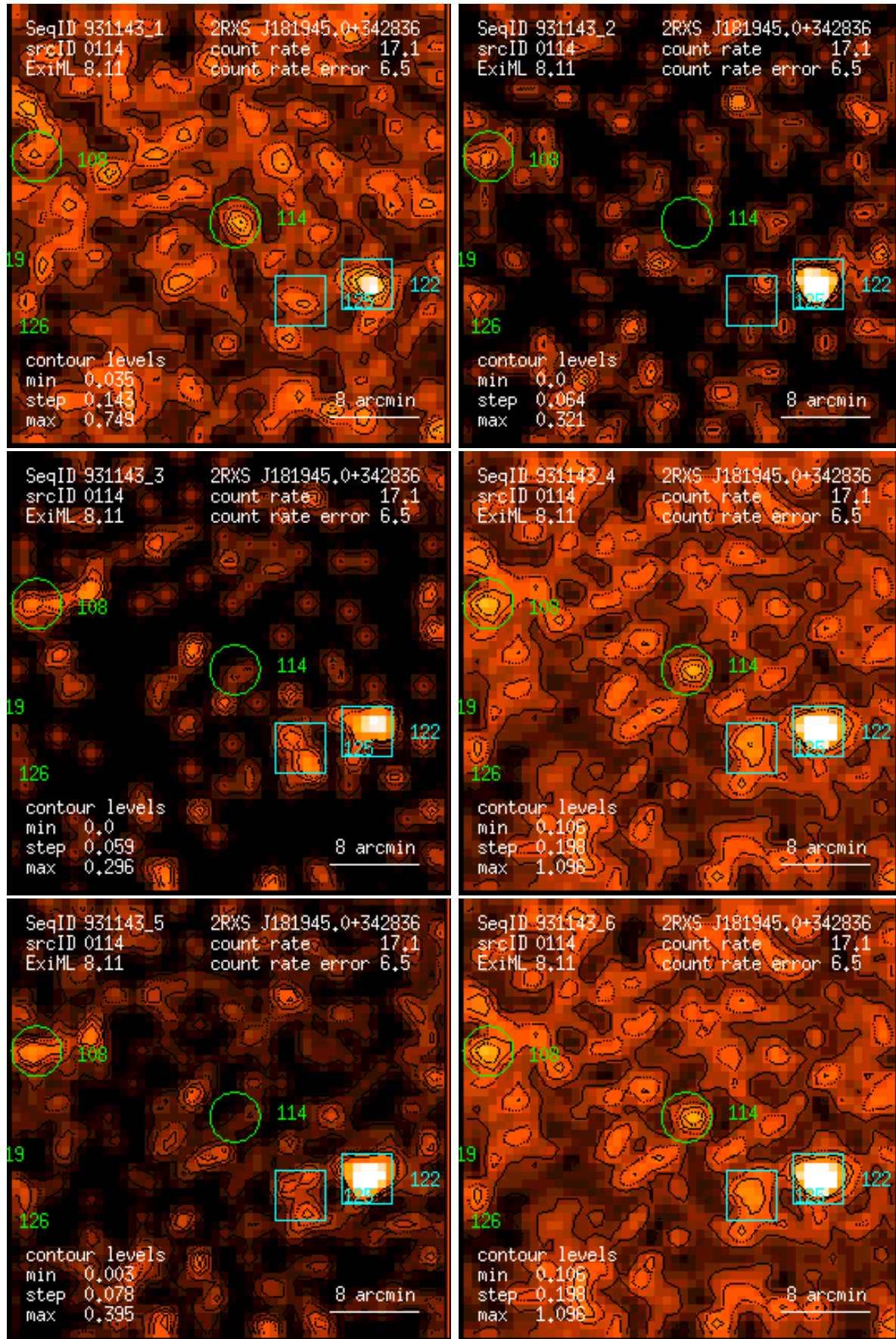
Figure 114: RASS 931143: detection 0114: band rate images, Gaussian filter: (1) PSPC channels 11 – 41, (2) 52 – 90, (3) 91 – 201, (4) 11 – 235, (5) 52 – 201, (6) 11 – 201. Broad band rates in counts/ks. Band rate contour levels in counts/ks/arcmin 2 .
