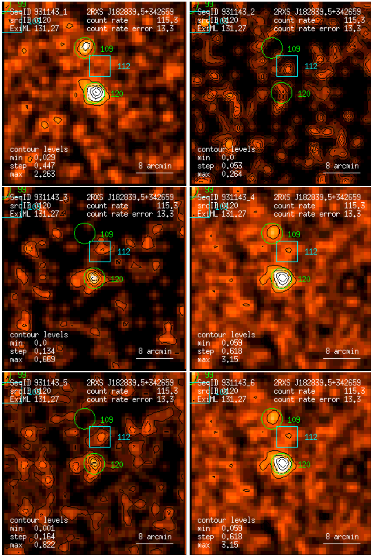
Figure 120: RASS 931143: detection 0120: band rate images, Gaussian filter: (1) PSPC channels 11 – 41, (2) 52 – 90, (3) 91 – 201, (4) 11 – 235, (5) 52 – 201, (6) 11 – 201. Broad band rates in counts/ks. Band rate contour levels in counts/ks/arcmin 2 .
