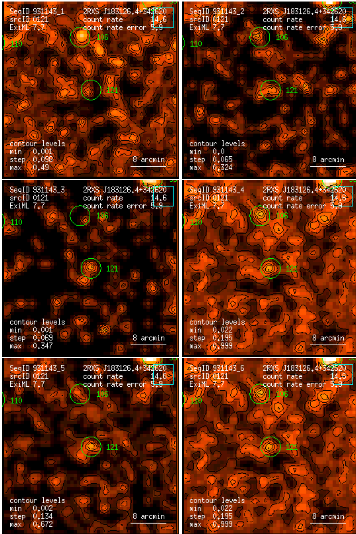
Figure 121: RASS 931143: detection 0121: band rate images, Gaussian filter: (1) PSPC channels 11 – 41, (2) 52 – 90, (3) 91 – 201, (4) 11 – 235, (5) 52 – 201, (6) 11 – 201. Broad band rates in counts/ks. Band rate contour levels in counts/ks/arcmin 2 .
