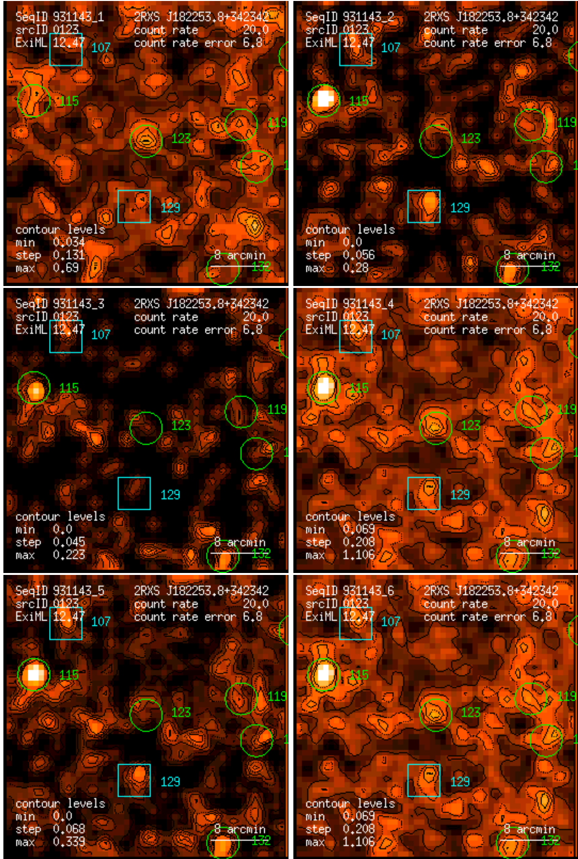
Figure 123: RASS 931143: detection 0123: band rate images, Gaussian filter: (1) PSPC channels 11 – 41, (2) 52 – 90, (3) 91 – 201, (4) 11 – 235, (5) 52 – 201, (6) 11 – 201. Broad band rates in counts/ks. Band rate contour levels in counts/ks/arcmin 2 .
