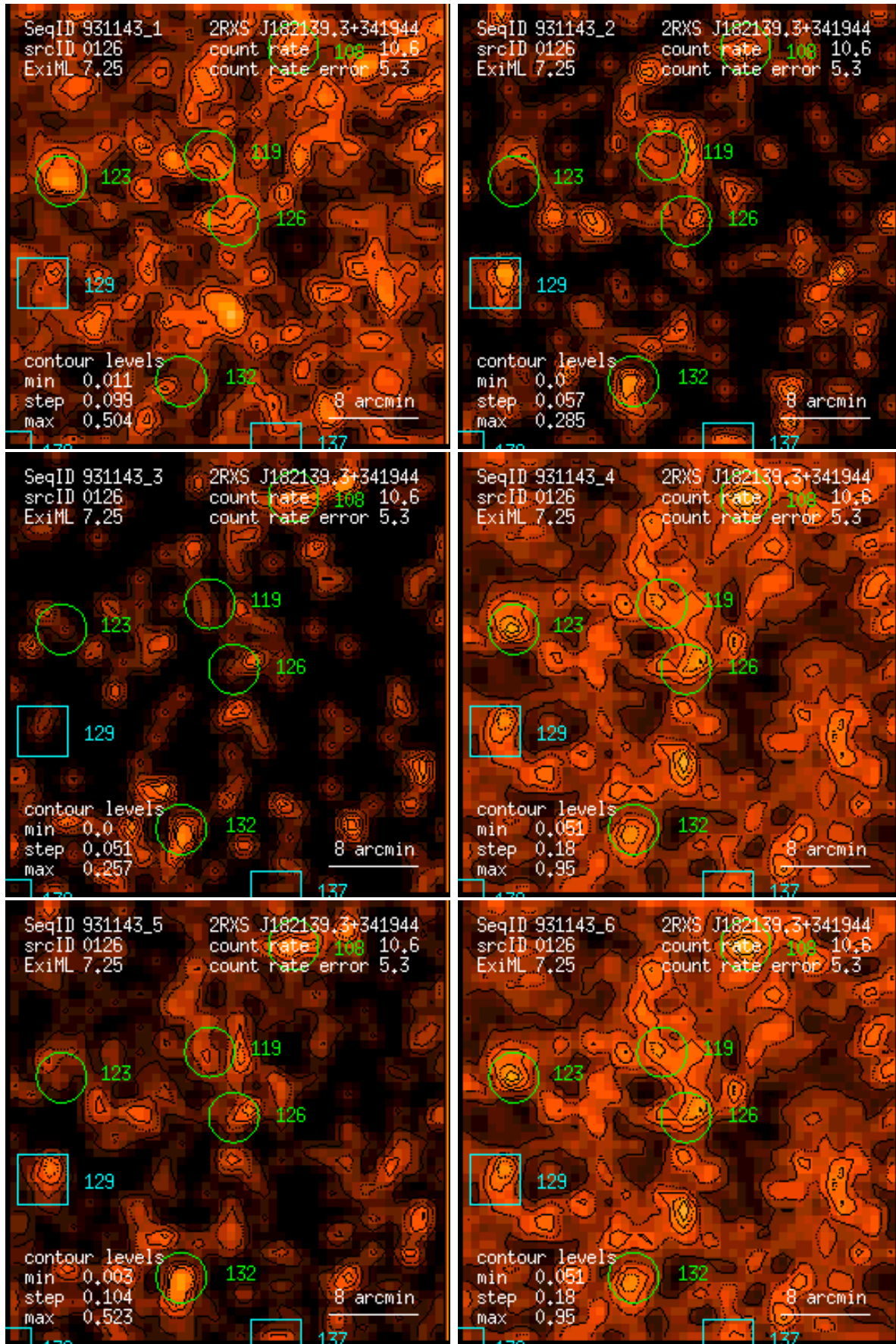
Figure 126: RASS 931143: detection 0126: band rate images, Gaussian filter: (1) PSPC channels 11 – 41, (2) 52 – 90, (3) 91 – 201, (4) 11 – 235, (5) 52 – 201, (6) 11 – 201. Broad band rates in counts/ks. Band rate contour levels in counts/ks/arcmin 2 .
