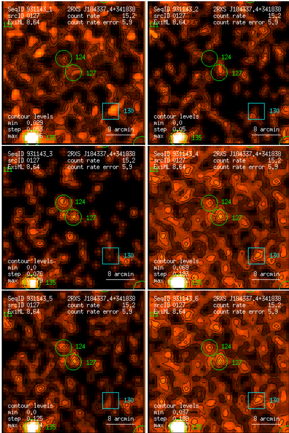
Figure 127: RASS 931143: detection 0127: band rate images, Gaussian filter: (1) PSPC channels 11 – 41, (2) 52 – 90, (3) 91 – 201, (4) 11 – 235, (5) 52 – 201, (6) 11 – 201. Broad band rates in counts/ks. Band rate contour levels in counts/ks/arcmin 2 .
