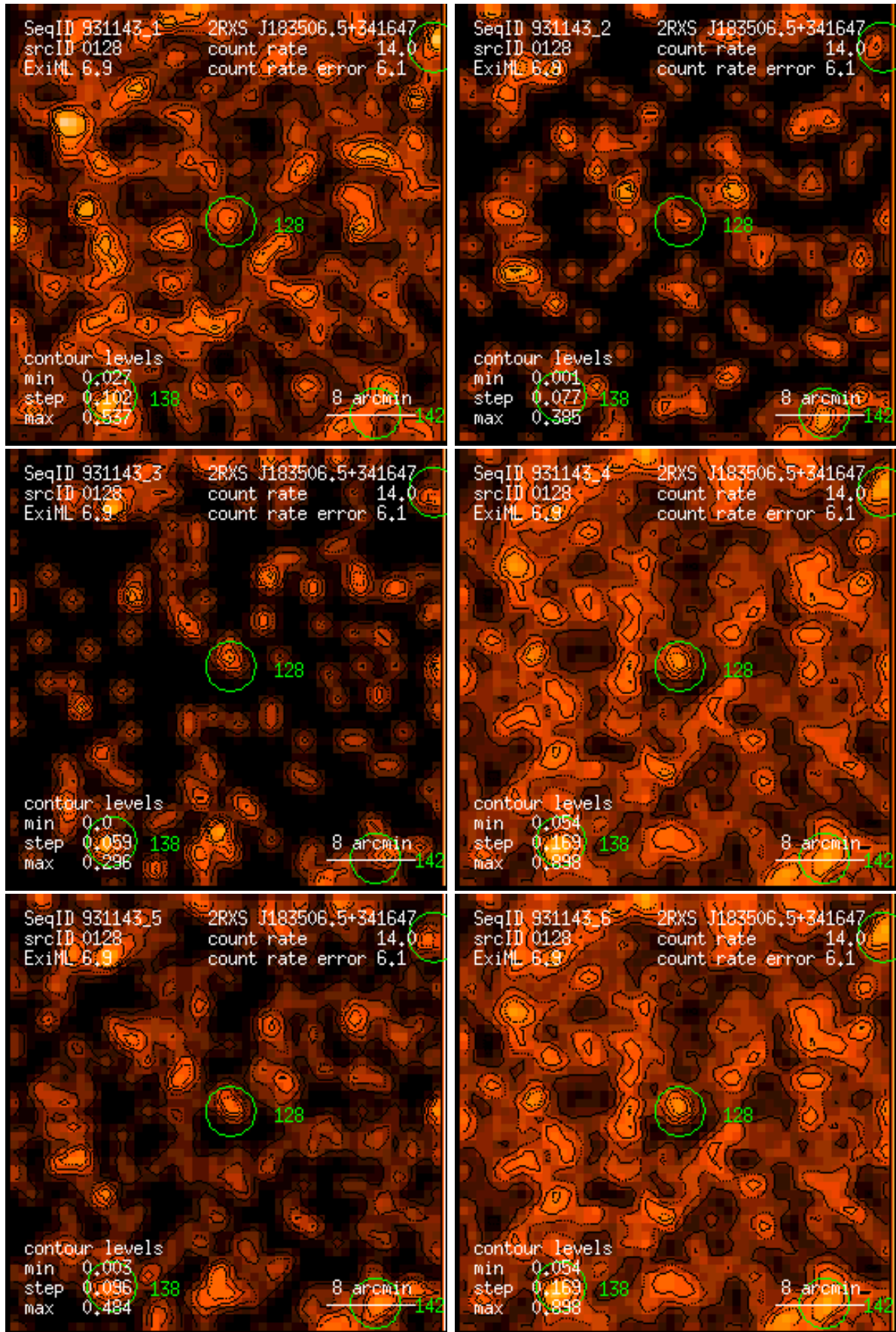
Figure 128: RASS 931143: detection 0128: band rate images, Gaussian filter: (1) PSPC channels 11 – 41, (2) 52 – 90, (3) 91 – 201, (4) 11 – 235, (5) 52 – 201, (6) 11 – 201. Broad band rates in counts/ks. Band rate contour levels in counts/ks/arcmin 2 .
