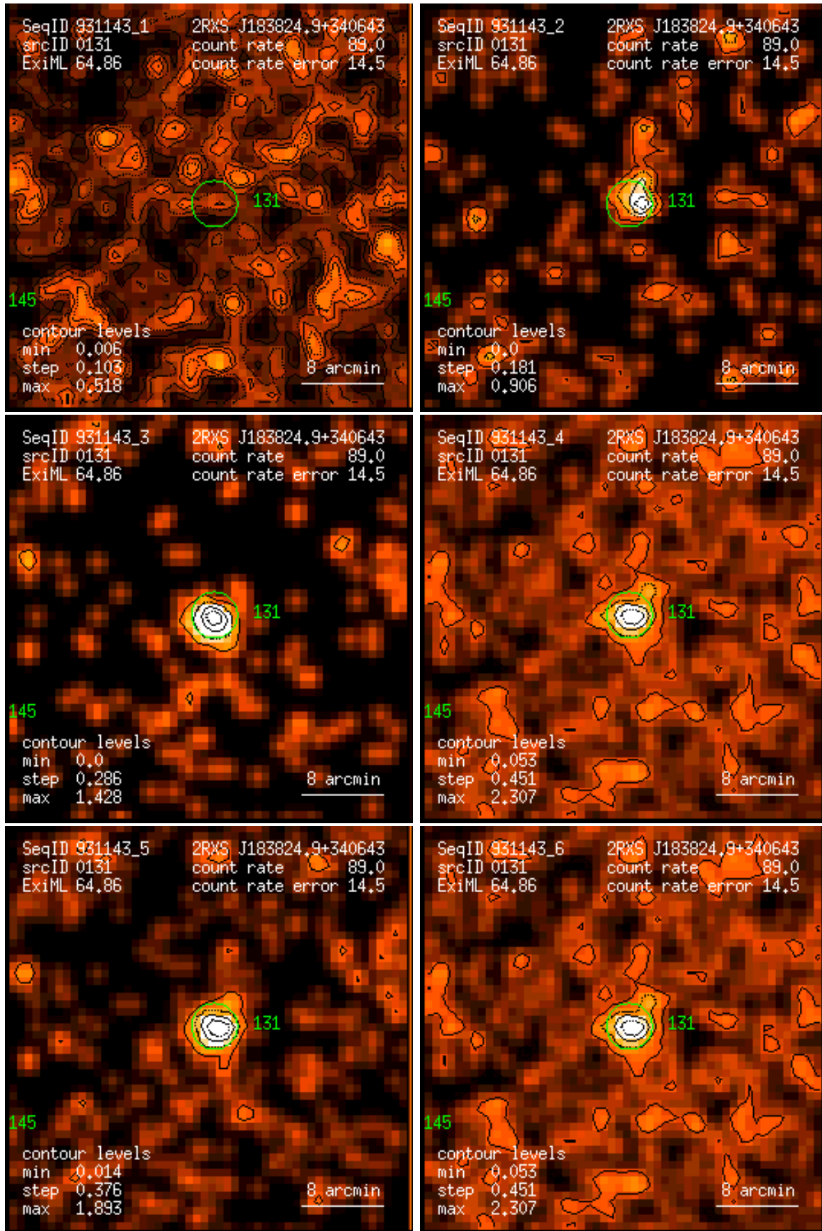
Figure 131: RASS 931143: detection 0131: band rate images, Gaussian filter: (1) PSPC channels 11 – 41, (2) 52 – 90, (3) 91 – 201, (4) 11 – 235, (5) 52 – 201, (6) 11 – 201. Broad band rates in counts/ks. Band rate contour levels in counts/ks/arcmin 2 .
