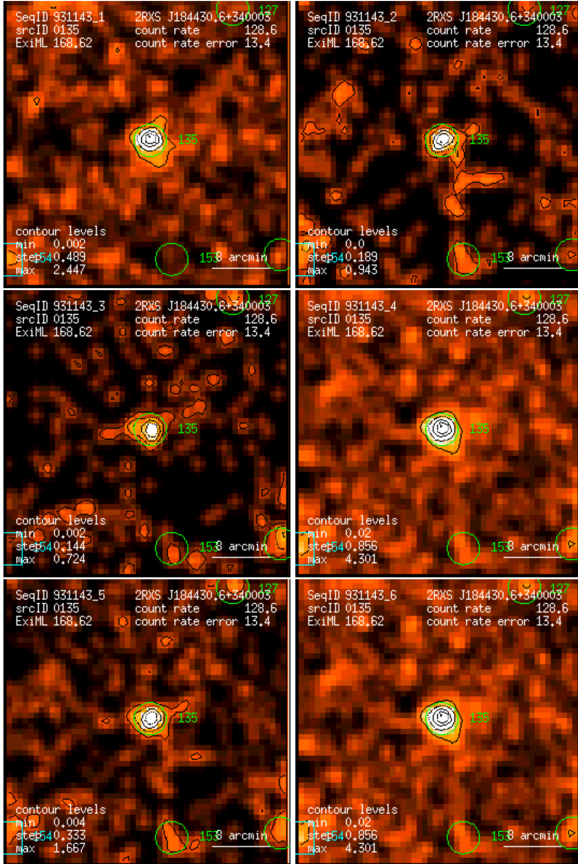
Figure 135: RASS 931143: detection 0135: band rate images, Gaussian filter: (1) PSPC channels 11 – 41, (2) 52 – 90, (3) 91 – 201, (4) 11 – 235, (5) 52 – 201, (6) 11 – 201. Broad band rates in counts/ks. Band rate contour levels in counts/ks/arcmin 2 .
