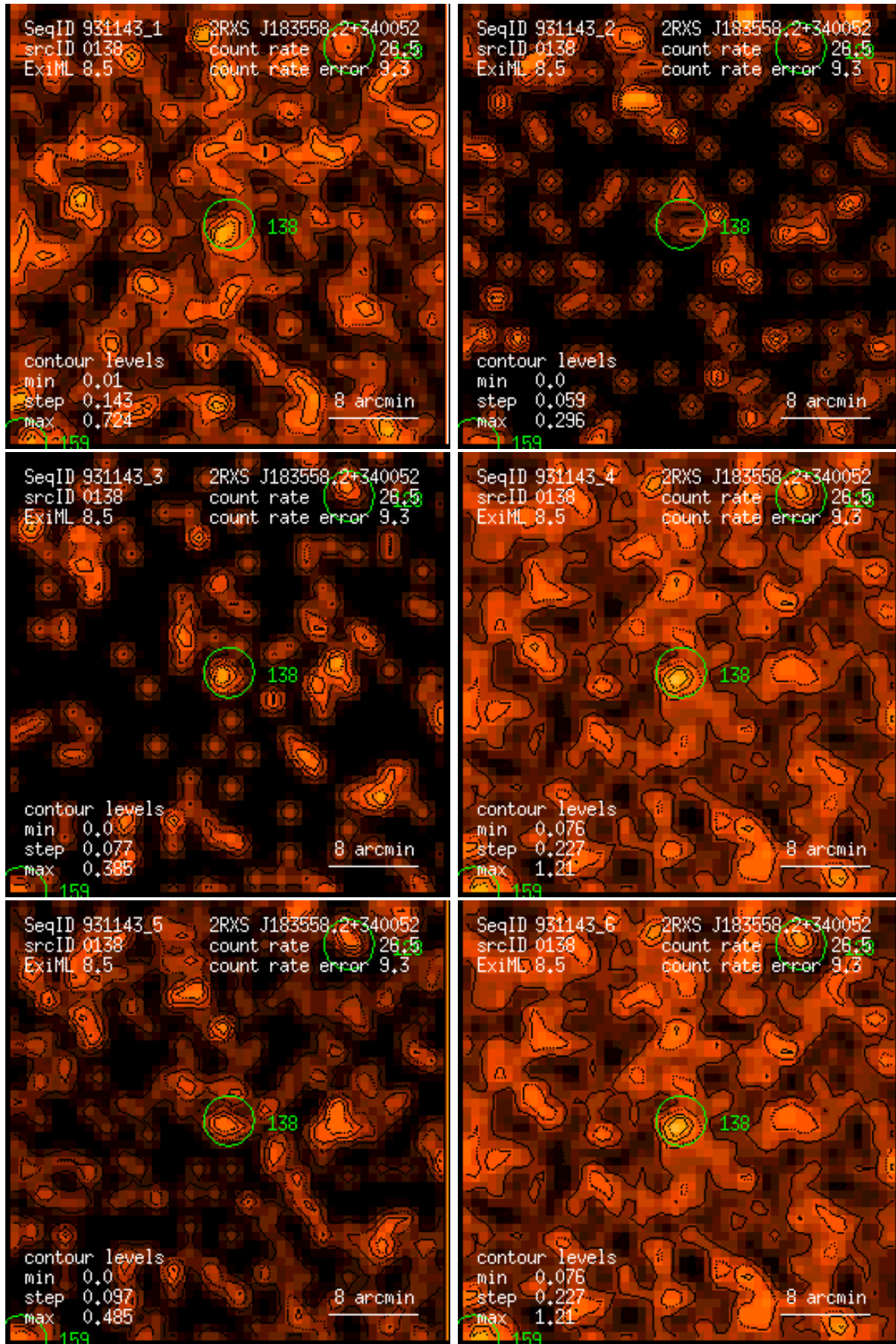
Figure 138: RASS 931143: detection 0138: band rate images, Gaussian filter: (1) PSPC channels 11 – 41, (2) 52 – 90, (3) 91 – 201, (4) 11 – 235, (5) 52 – 201, (6) 11 – 201. Broad band rates in counts/ks. Band rate contour levels in counts/ks/arcmin 2 .
