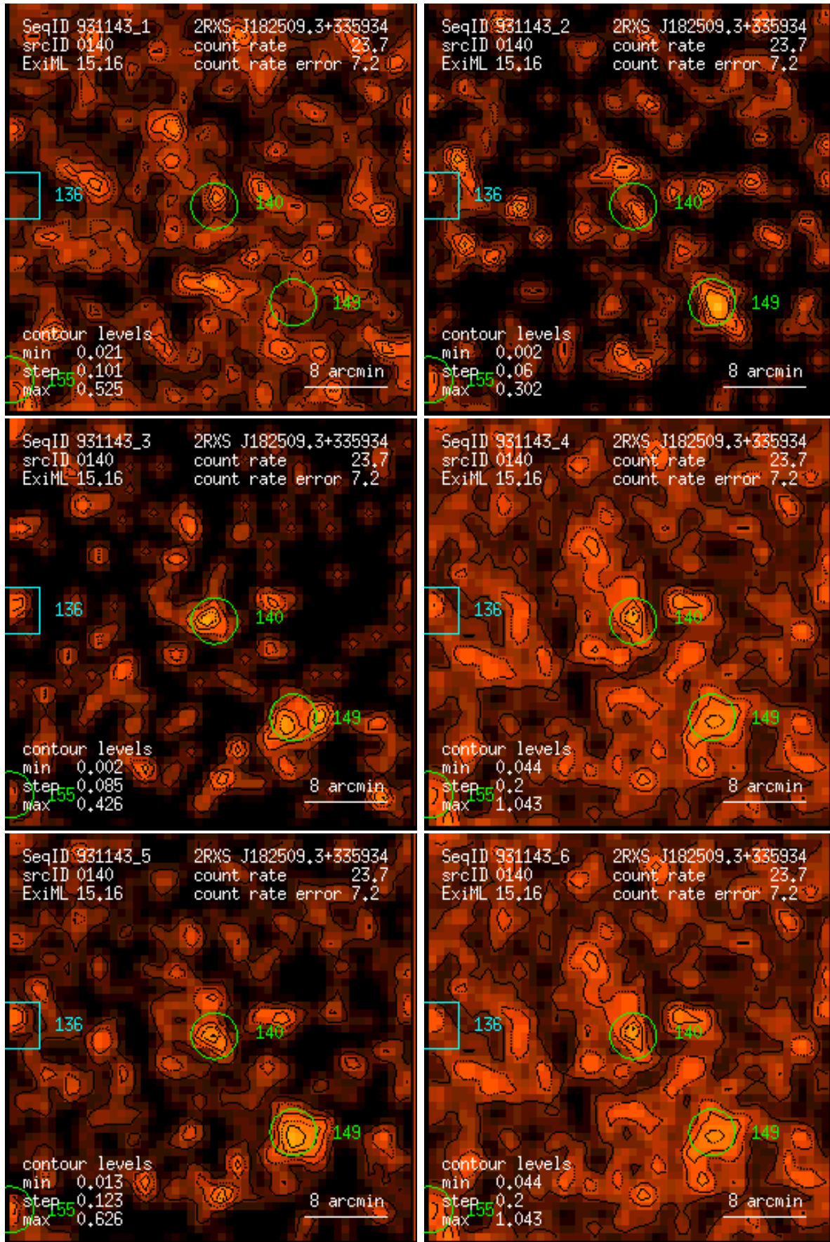
Figure 140: RASS 931143: detection 0140: band rate images, Gaussian filter: (1) PSPC channels 11 – 41, (2) 52 – 90, (3) 91 – 201, (4) 11 – 235, (5) 52 – 201, (6) 11 – 201. Broad band rates in counts/ks. Band rate contour levels in counts/ks/arcmin 2 .
