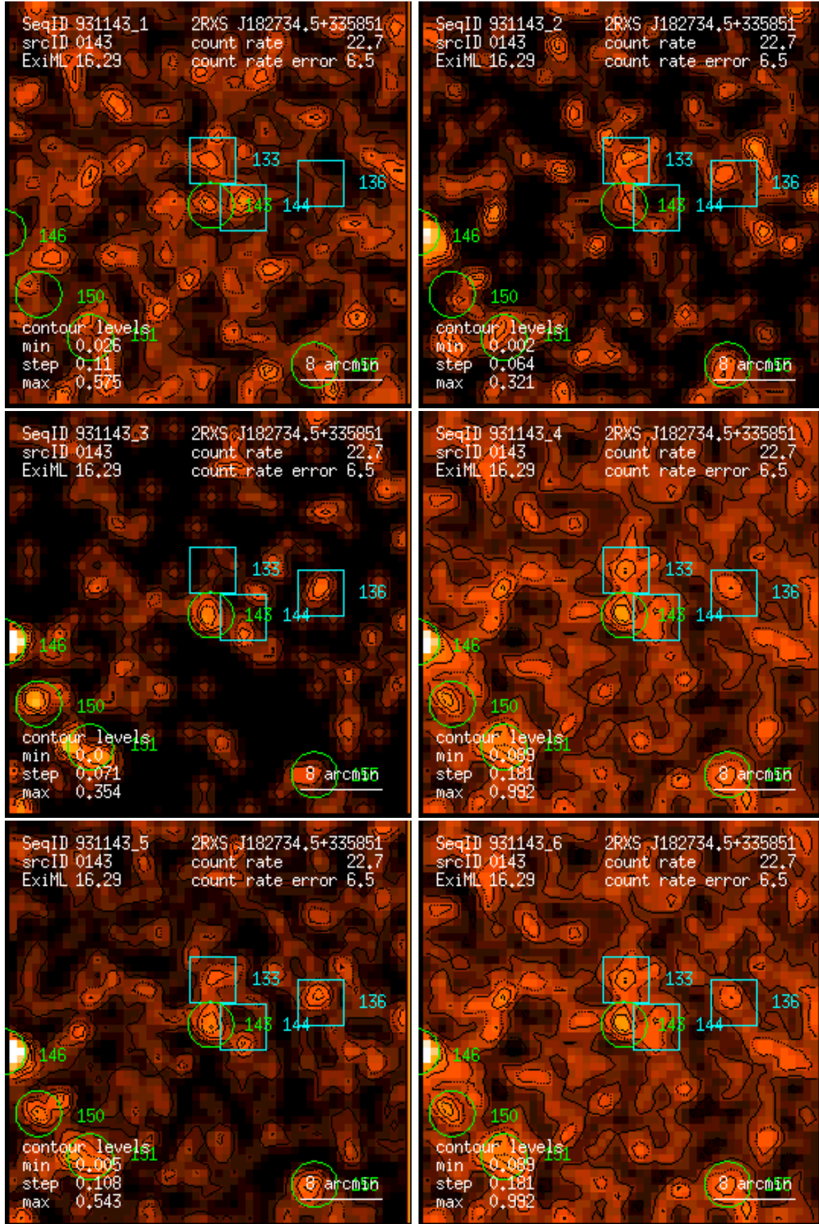
Figure 143: RASS 931143: detection 0143: band rate images, Gaussian filter: (1) PSPC channels 11 – 41, (2) 52 – 90, (3) 91 – 201, (4) 11 – 235, (5) 52 – 201, (6) 11 – 201. Broad band rates in counts/ks. Band rate contour levels in counts/ks/arcmin 2 .
