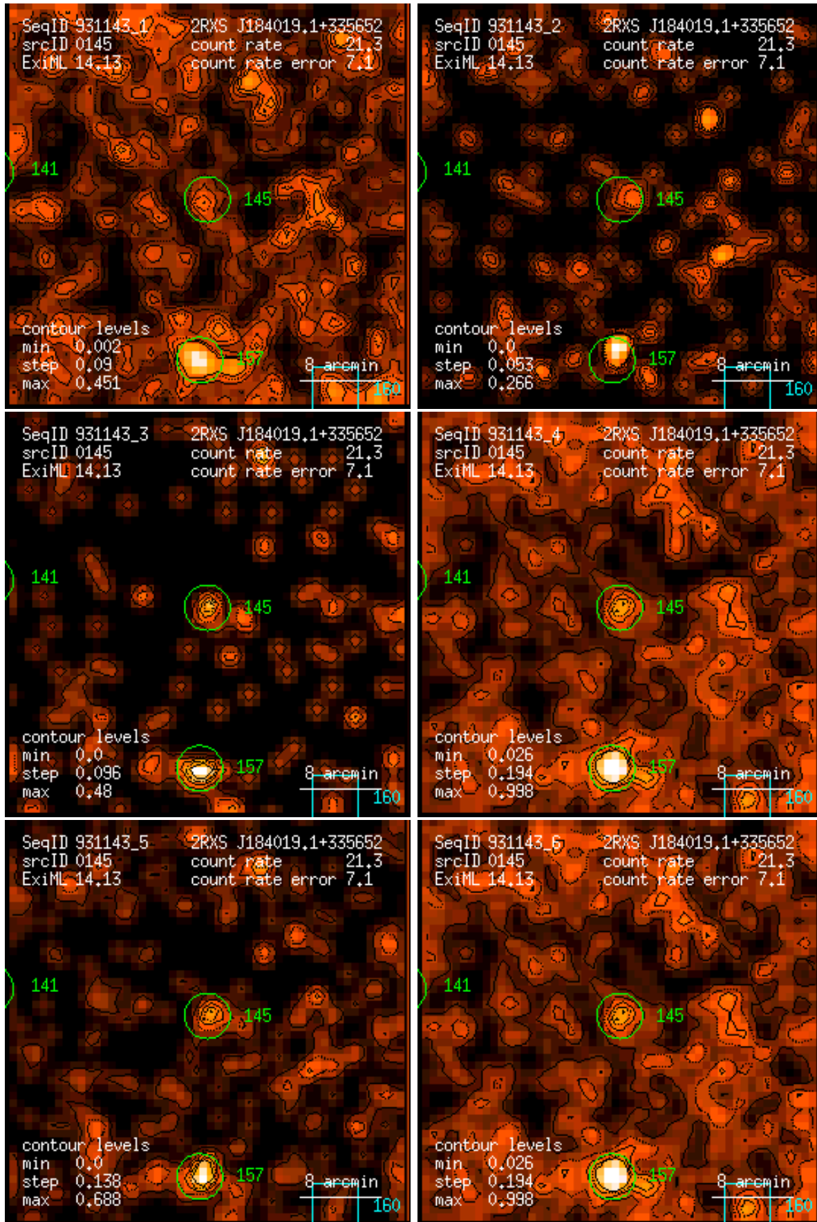
Figure 145: RASS 931143: detection 0145: band rate images, Gaussian filter: (1) PSPC channels 11 – 41, (2) 52 – 90, (3) 91 – 201, (4) 11 – 235, (5) 52 – 201, (6) 11 – 201. Broad band rates in counts/ks. Band rate contour levels in counts/ks/arcmin 2 .
