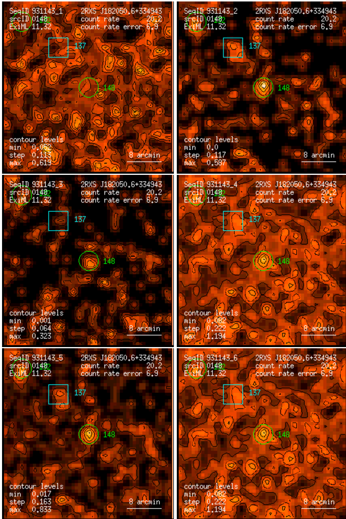
Figure 148: RASS 931143: detection 0148: band rate images, Gaussian filter: (1) PSPC channels 11 – 41, (2) 52 – 90, (3) 91 – 201, (4) 11 – 235, (5) 52 – 201, (6) 11 – 201. Broad band rates in counts/ks. Band rate contour levels in counts/ks/arcmin 2 .
