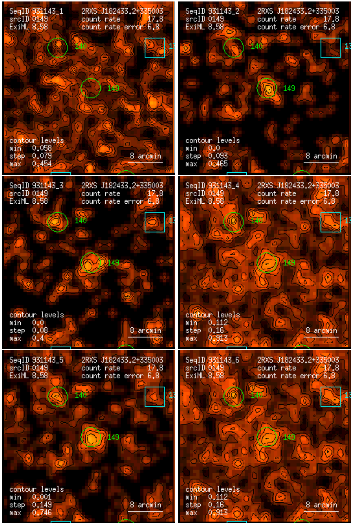
Figure 149: RASS 931143: detection 0149: band rate images, Gaussian filter: (1) PSPC channels 11 – 41, (2) 52 – 90, (3) 91 – 201, (4) 11 – 235, (5) 52 – 201, (6) 11 – 201. Broad band rates in counts/ks. Band rate contour levels in counts/ks/arcmin 2 .
