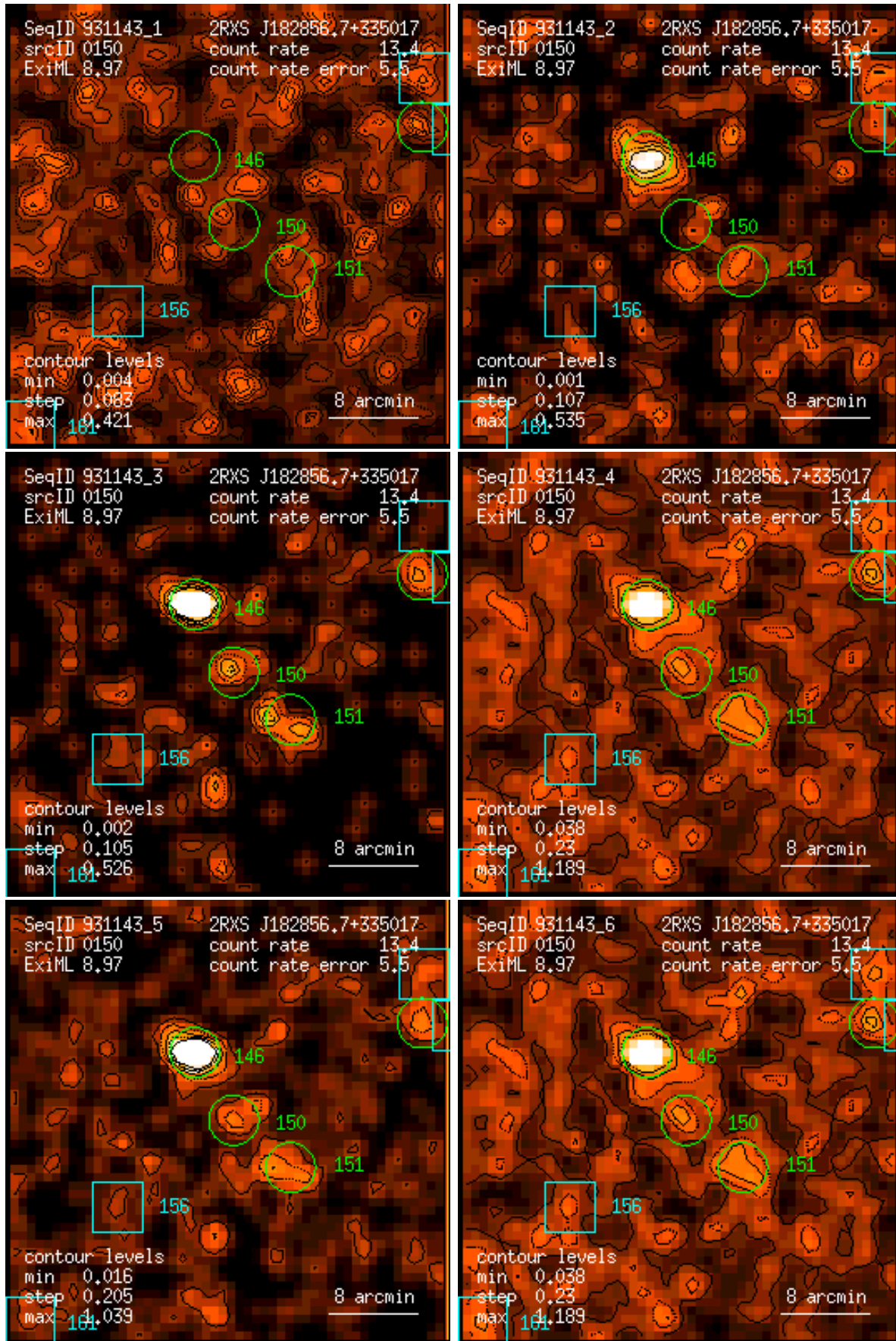
Figure 150: RASS 931143: detection 0150: band rate images, Gaussian filter: (1) PSPC channels 11 – 41, (2) 52 – 90, (3) 91 – 201, (4) 11 – 235, (5) 52 – 201, (6) 11 – 201. Broad band rates in counts/ks. Band rate contour levels in counts/ks/arcmin 2 .
