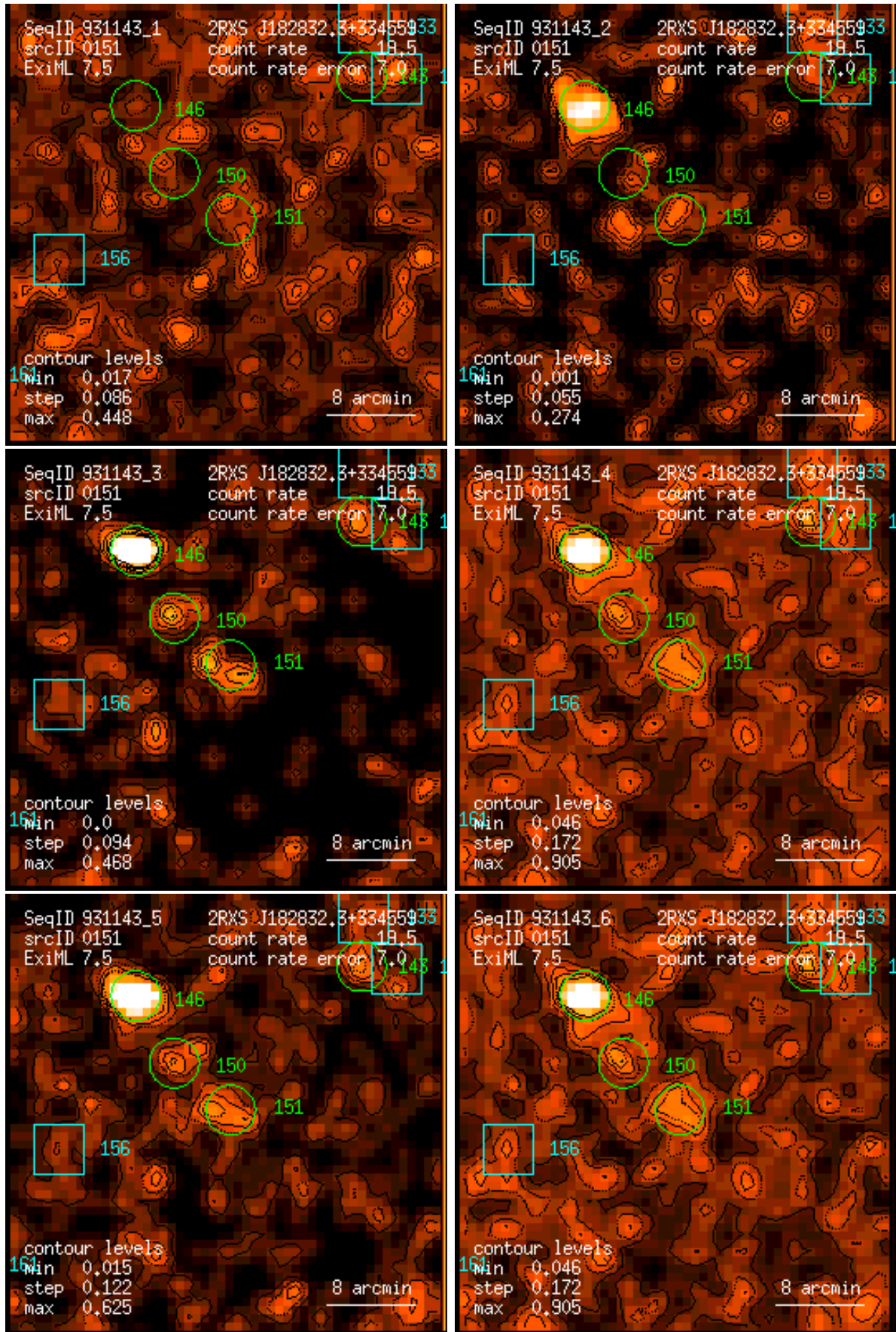
Figure 151: RASS 931143: detection 0151: band rate images, Gaussian filter: (1) PSPC channels 11 – 41, (2) 52 – 90, (3) 91 – 201, (4) 11 – 235, (5) 52 – 201, (6) 11 – 201. Broad band rates in counts/ks. Band rate contour levels in counts/ks/arcmin 2 .
