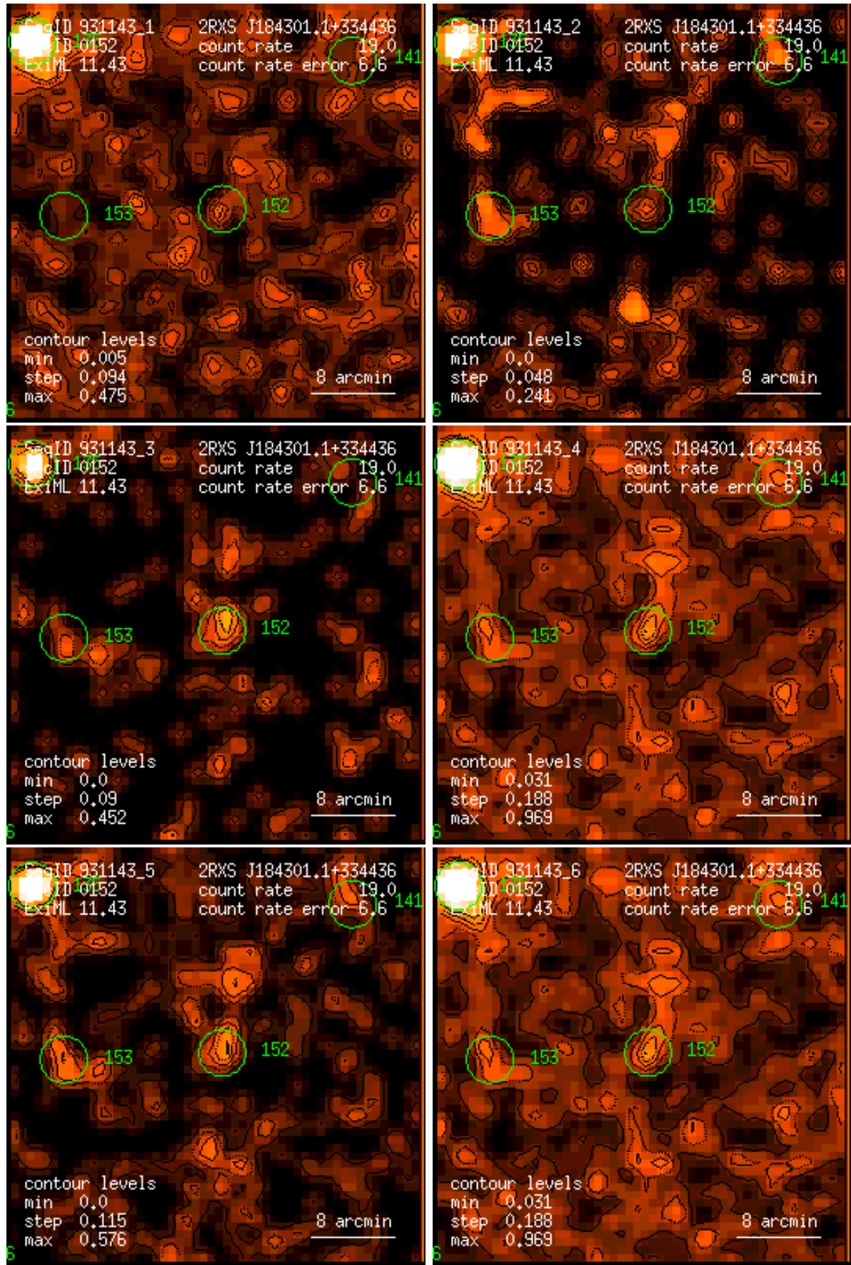
Figure 152: RASS 931143: detection 0152: band rate images, Gaussian filter: (1) PSPC channels 11 – 41, (2) 52 – 90, (3) 91 – 201, (4) 11 – 235, (5) 52 – 201, (6) 11 – 201. Broad band rates in counts/ks. Band rate contour levels in counts/ks/arcmin 2 .
