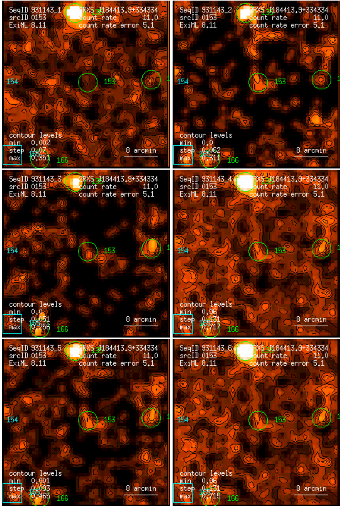
Figure 153: RASS 931143: detection 0153: band rate images, Gaussian filter: (1) PSPC channels 11 – 41, (2) 52 – 90, (3) 91 – 201, (4) 11 – 235, (5) 52 – 201, (6) 11 – 201. Broad band rates in counts/ks. Band rate contour levels in counts/ks/arcmin 2 .
