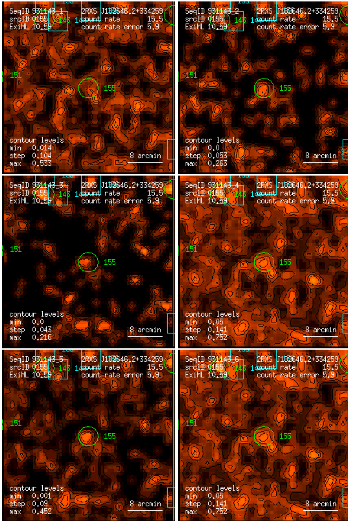
Figure 155: RASS 931143: detection 0155: band rate images, Gaussian filter: (1) PSPC channels 11 – 41, (2) 52 – 90, (3) 91 – 201, (4) 11 – 235, (5) 52 – 201, (6) 11 – 201. Broad band rates in counts/ks. Band rate contour levels in counts/ks/arcmin 2 .
