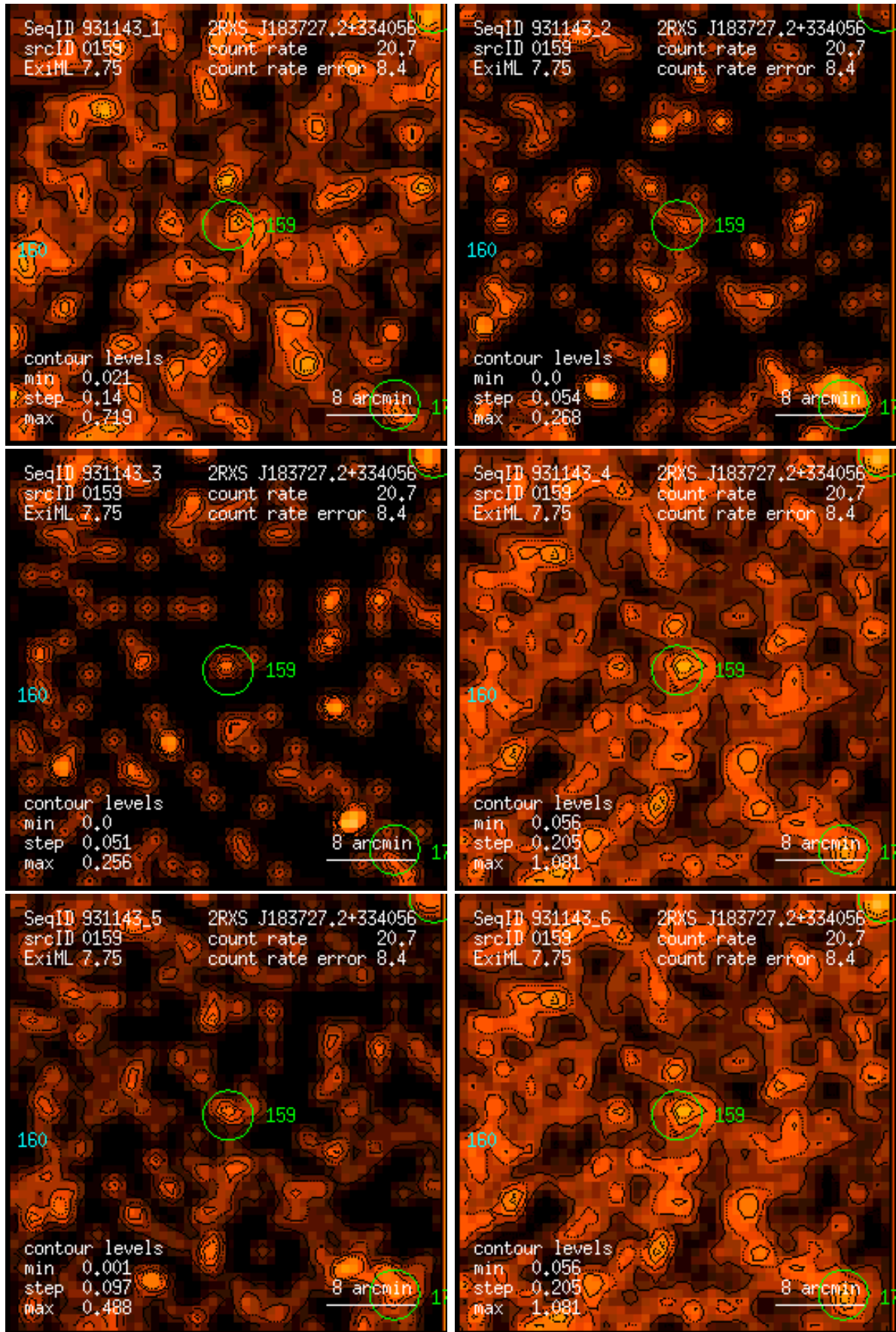
Figure 159: RASS 931143: detection 0159: band rate images, Gaussian filter: (1) PSPC channels 11 – 41, (2) 52 – 90, (3) 91 – 201, (4) 11 – 235, (5) 52 – 201, (6) 11 – 201. Broad band rates in counts/ks. Band rate contour levels in counts/ks/arcmin 2 .
