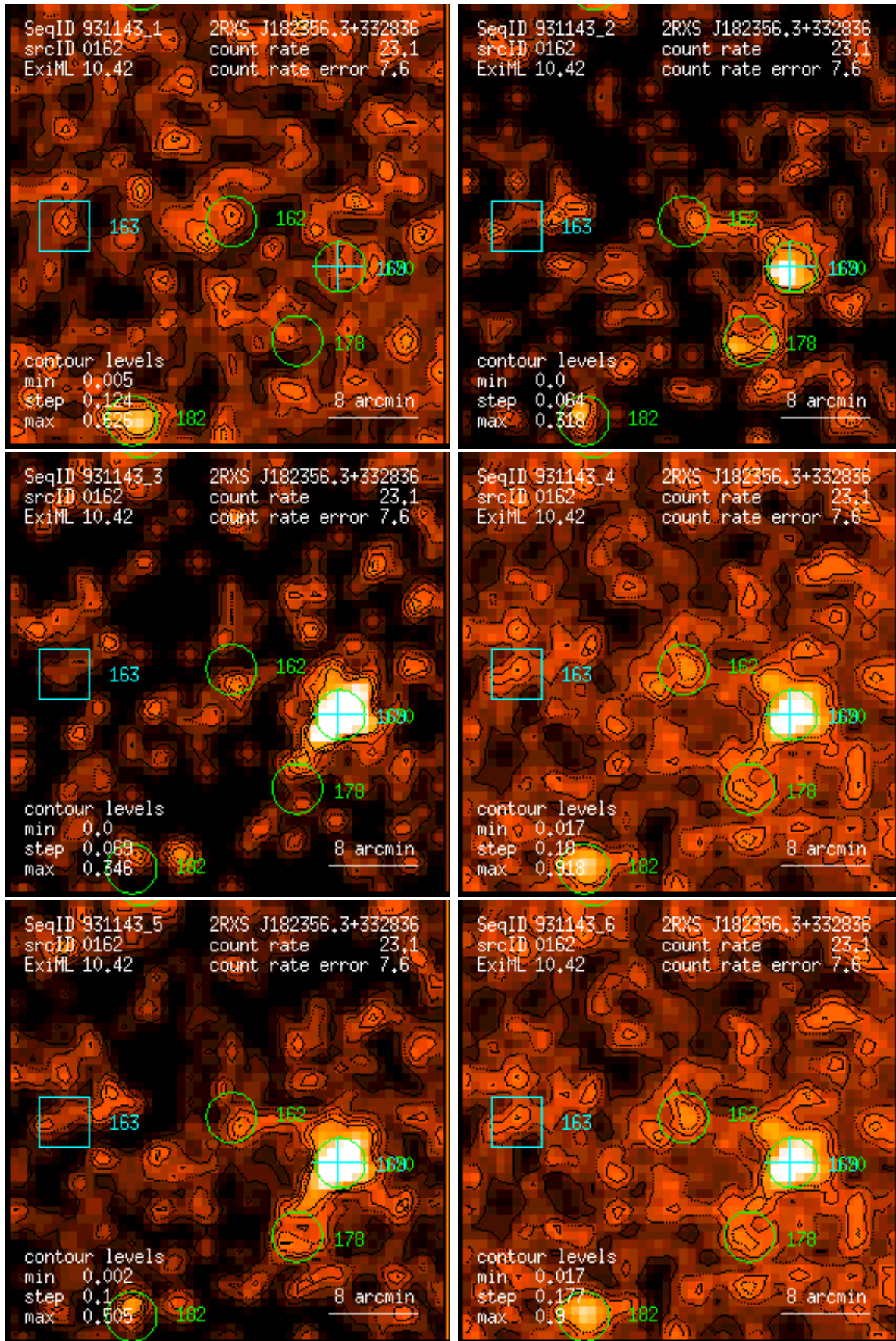
Figure 162: RASS 931143: detection 0162: band rate images, Gaussian filter: (1) PSPC channels 11 – 41, (2) 52 – 90, (3) 91 – 201, (4) 11 – 235, (5) 52 – 201, (6) 11 – 201. Broad band rates in counts/ks. Band rate contour levels in counts/ks/arcmin 2 .
